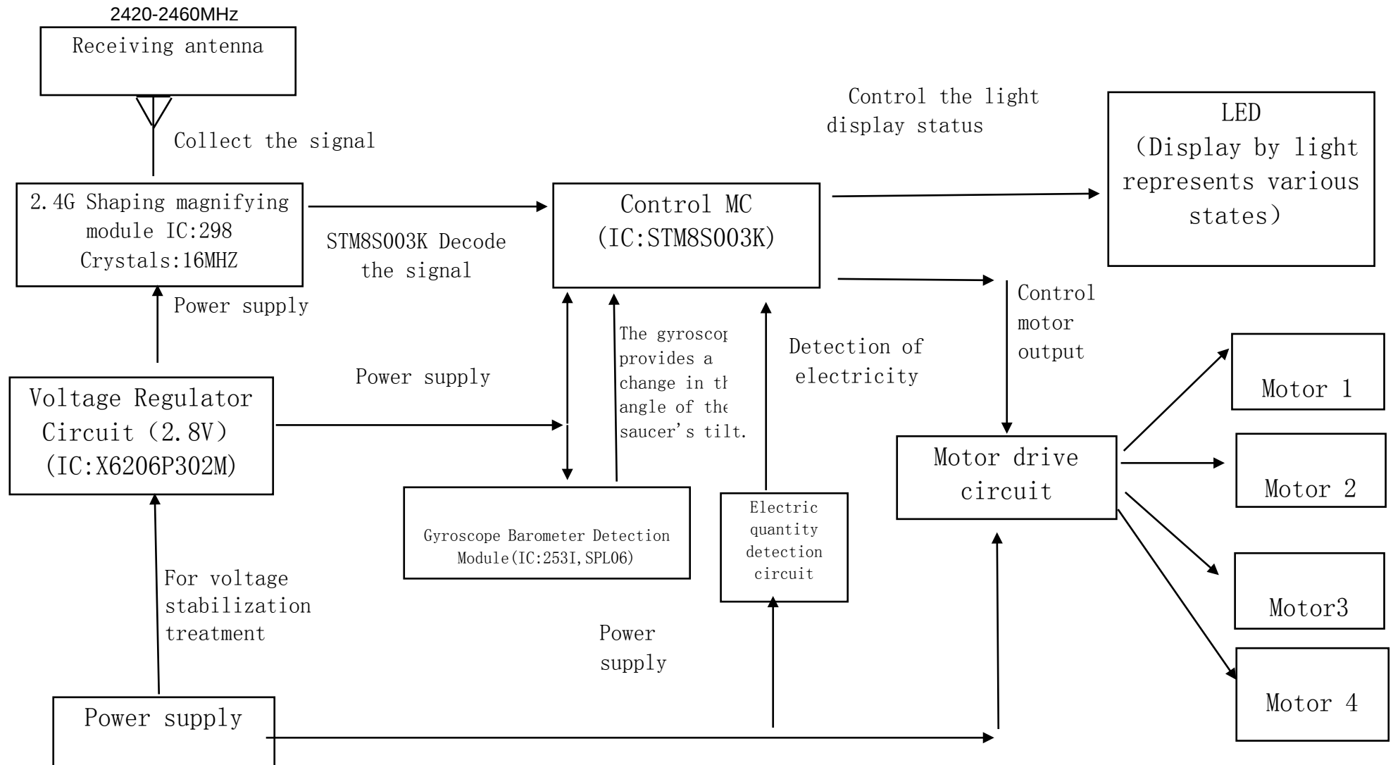
Block diagram of receiving principle
