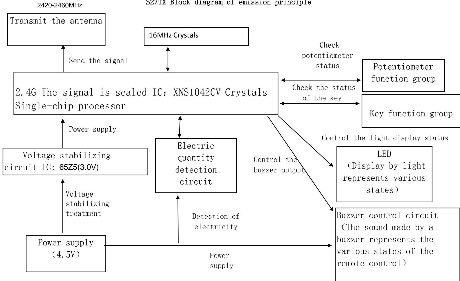
S27TX Block diagram of emission principle
