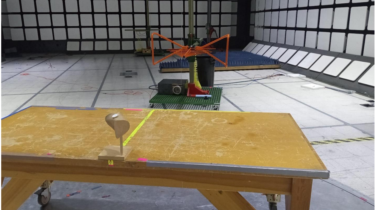
30 MHz – 1 GHz Test Setup
