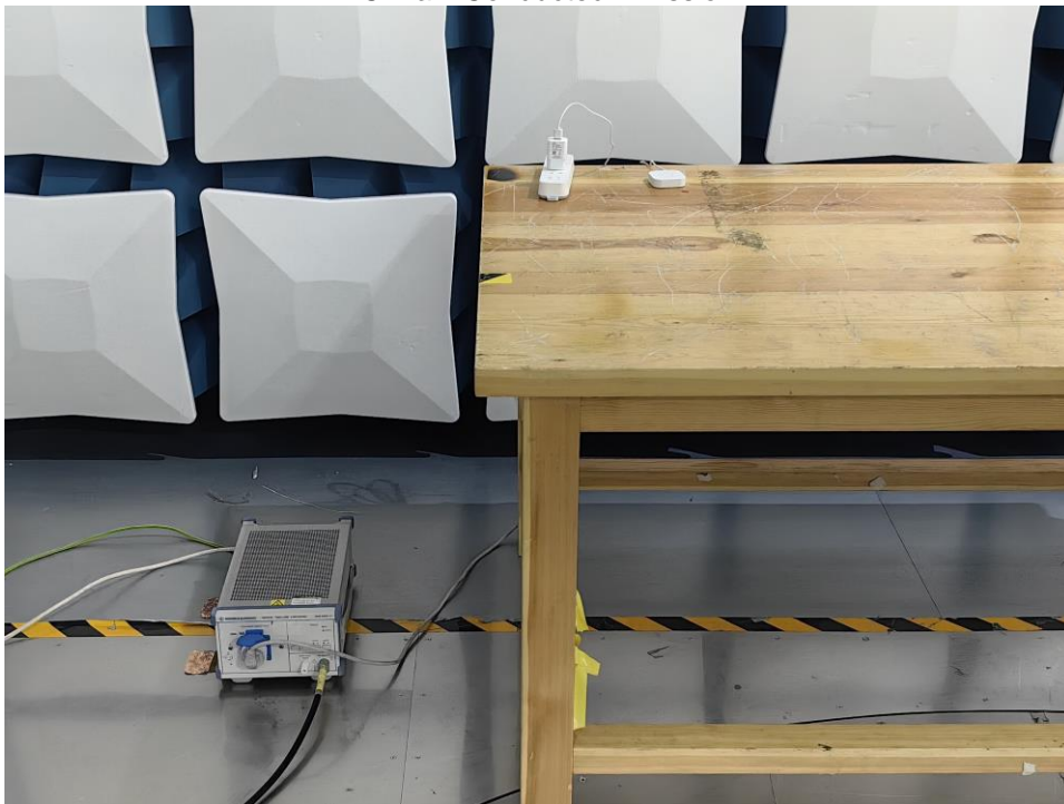
AC Main Conducted Emission
