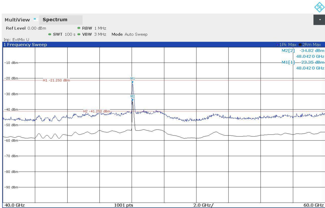
Plots No. 7: 40 GHz to 60 GHz, Horizontal / Vertical Polarization
