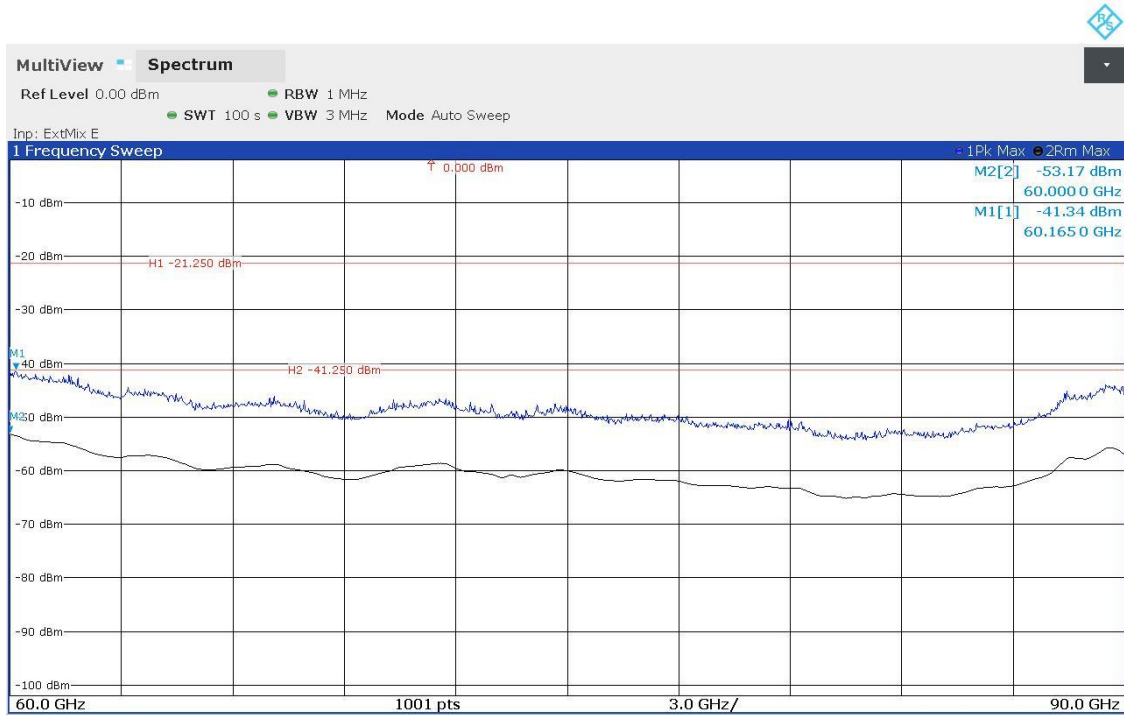
Plots No. 8: 60 GHz to 90 GHz, Horizontal / Vertical Polarization
