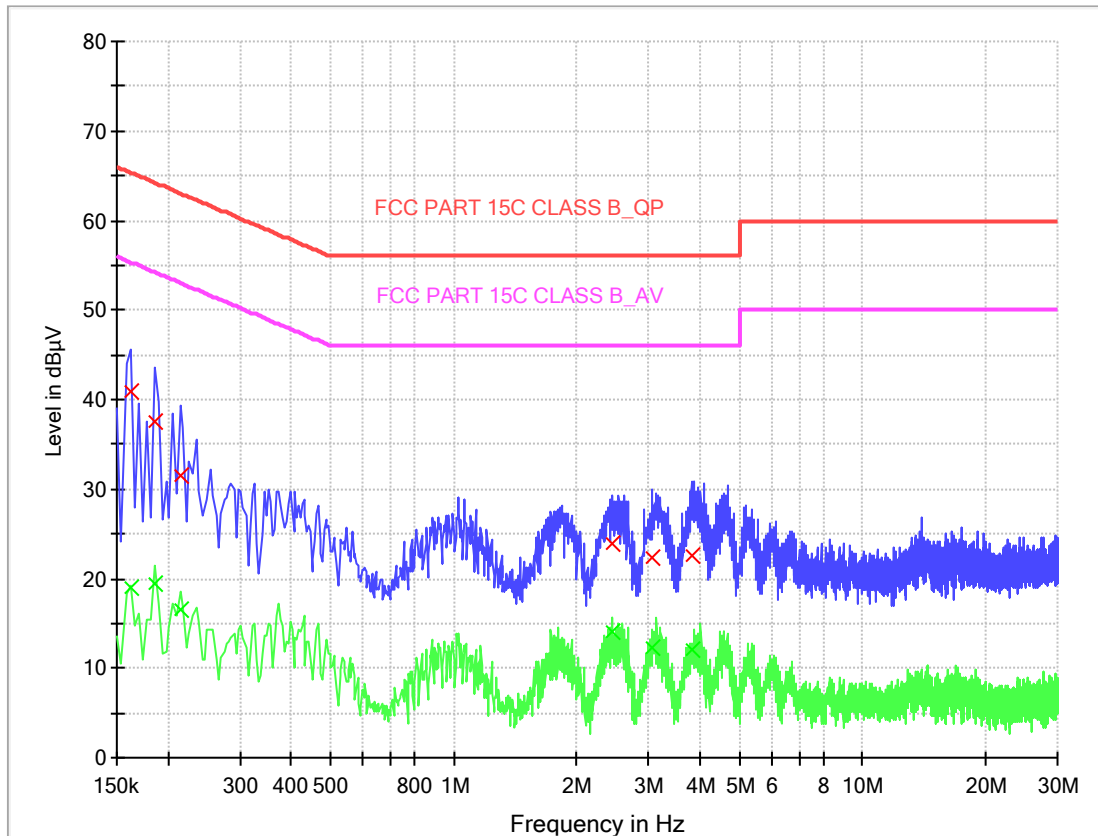
Plots No. 11: AC Mains Conducted Emission _ AC 120V/60Hz _ Neutral
