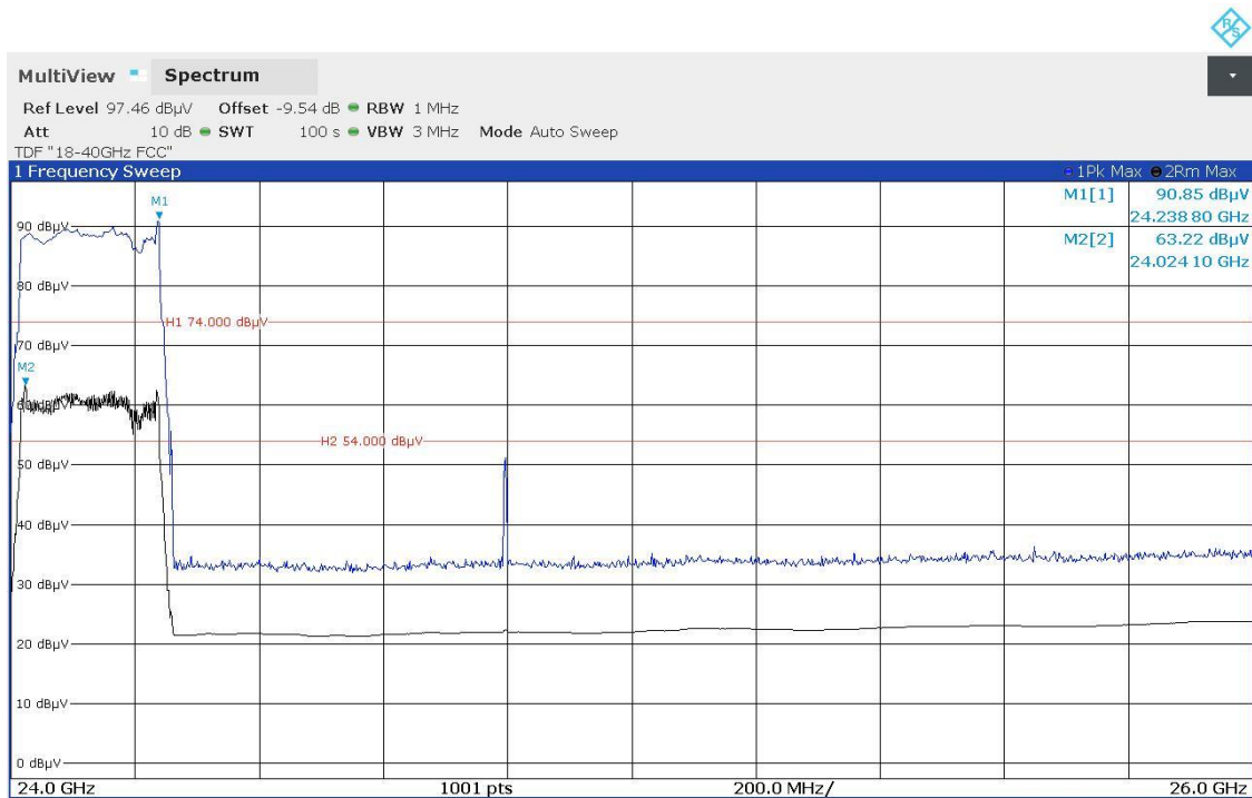
Plots No. 5: Radiated Higher Band-edge, Horizontal / Vertical Polarization
