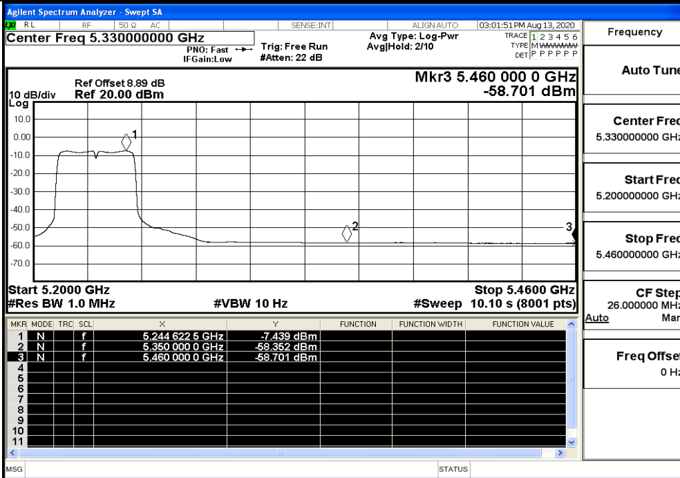
IEEE 802.11ac40 / Channel 48 / 5230MHz / Average
