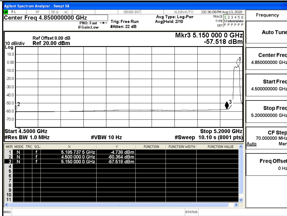
IEEE 802.11ac20 / Channel 36 / 5180MHz / Average
