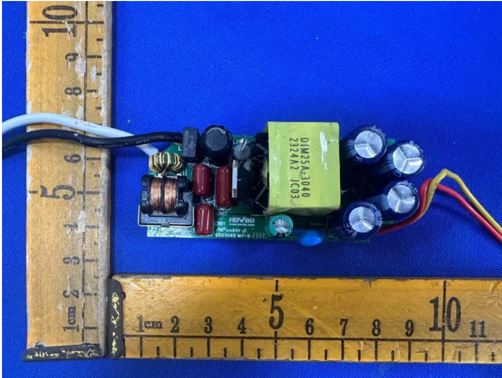
Fig.5(Model: VAN-SWR )
