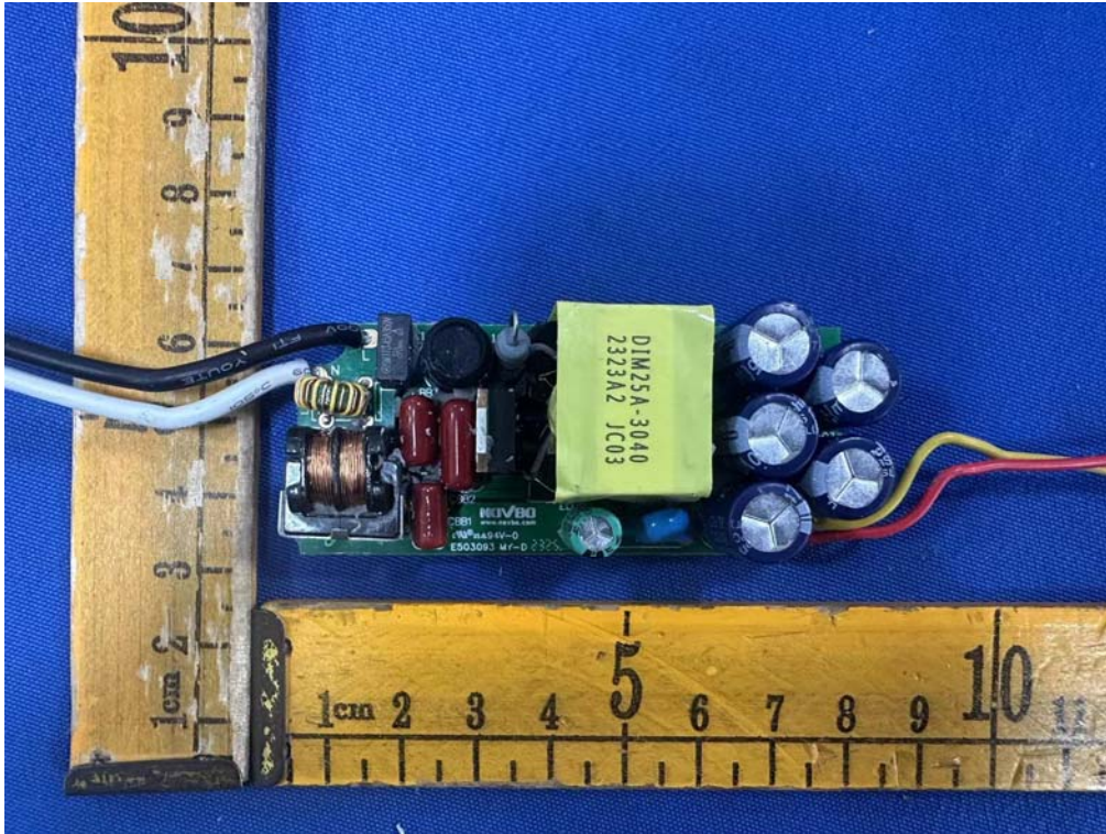
Fig.7(Model: VAN3-HOL5C )
