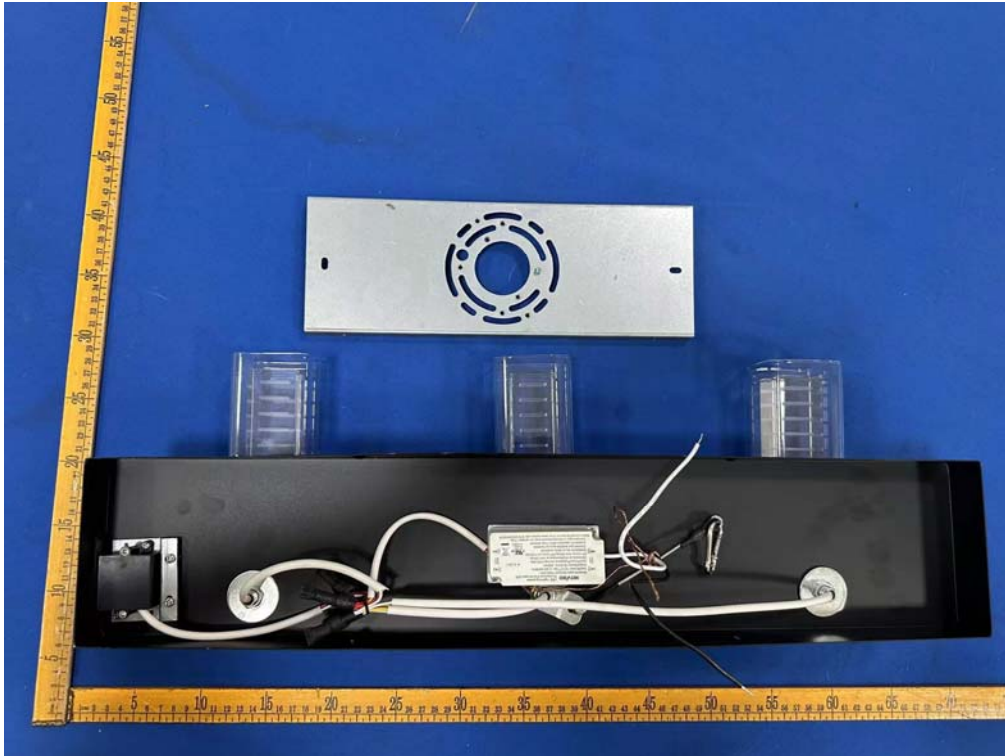
Fig.5(Model: VAN3-HOL5C )
