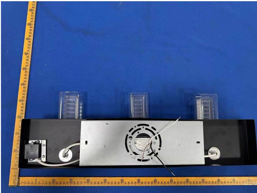
Fig.2(Model: VAN3-HOL5C )
