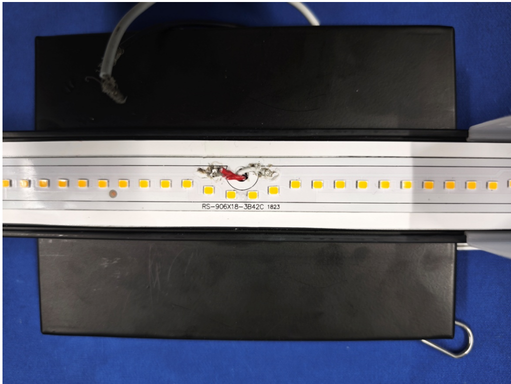
Fig.3(Model: V03045 )
