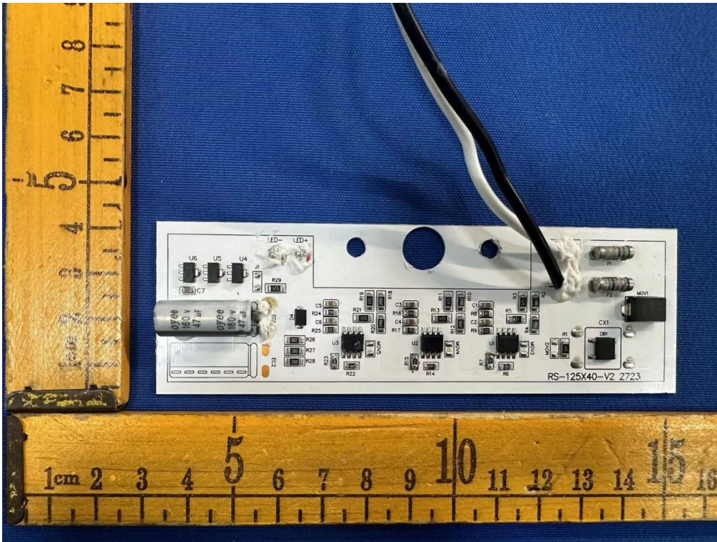
Fig.5(Model: V03045 )
