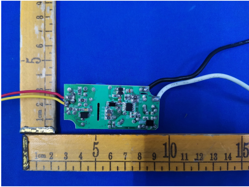
Fig.8(Model: TRK3-AL)
