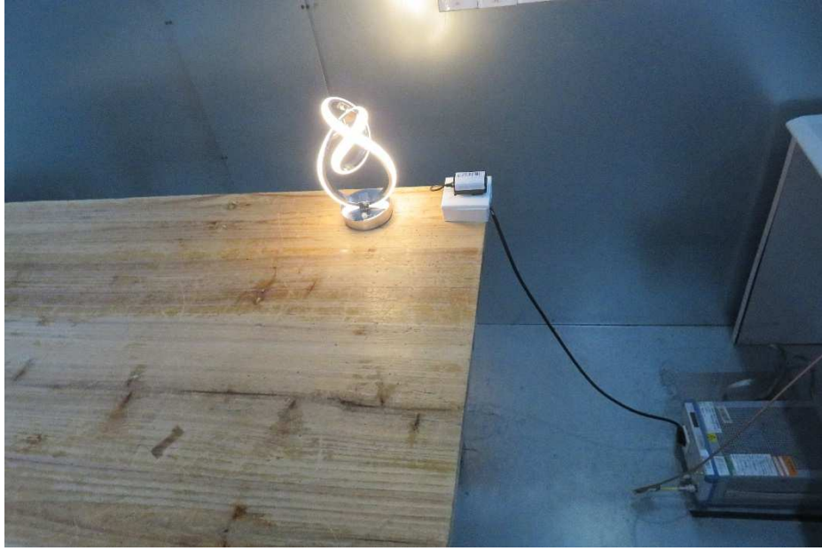
Conducted Emission
