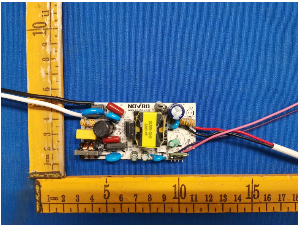
Fig.7 (Model:SCO-RIC)
