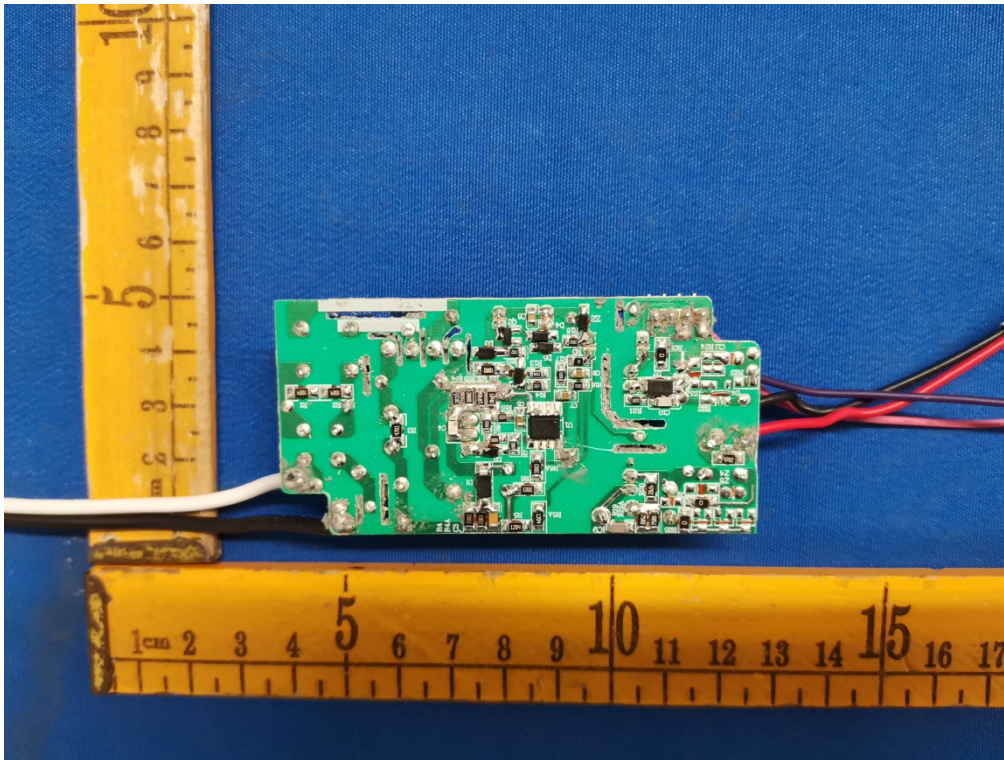
Fig.6 (Model:SCO-RIC)
