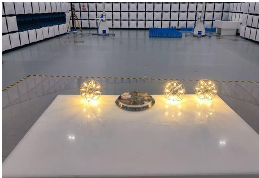
Radiated Disturbance below 1GHz
