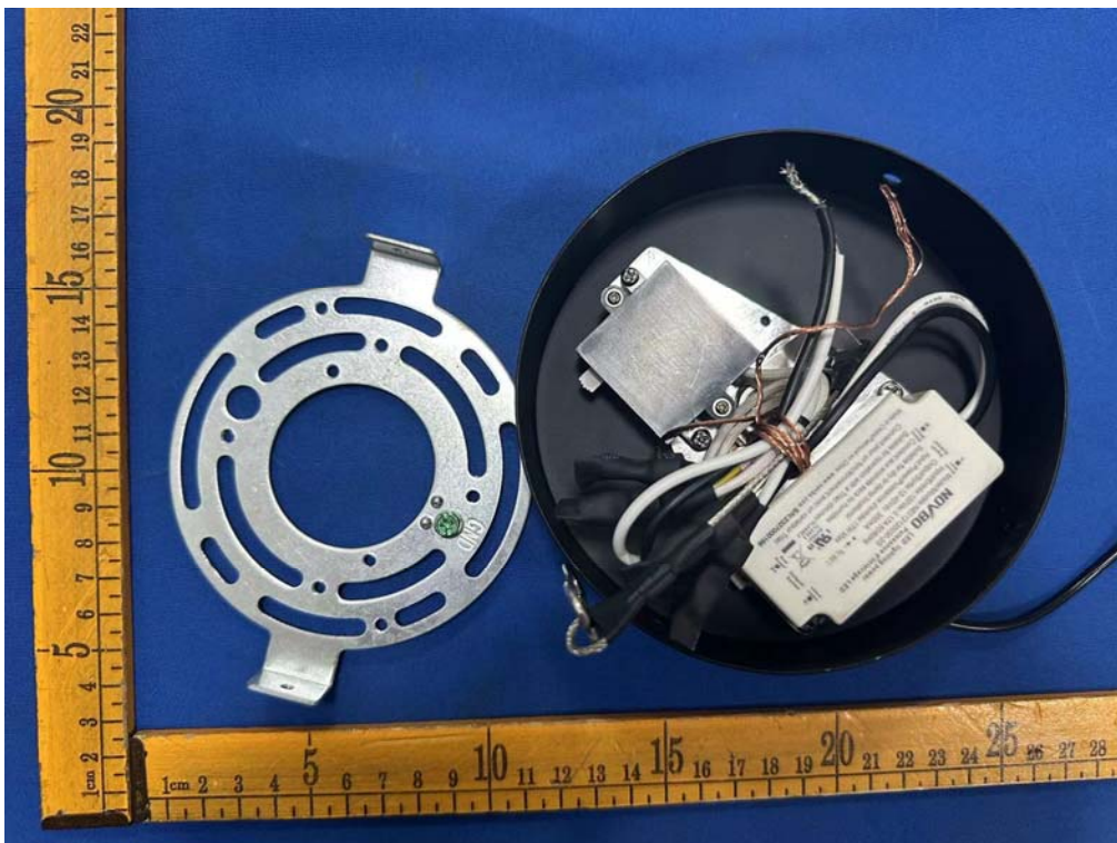
Fig.4(Model: PDT1-FI5C )
