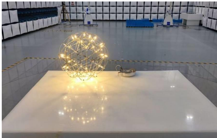
Radiated Disturbance below 1GHz
