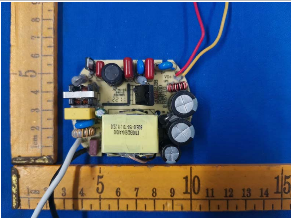
Fig.8(Model: PDT-AD5C)
