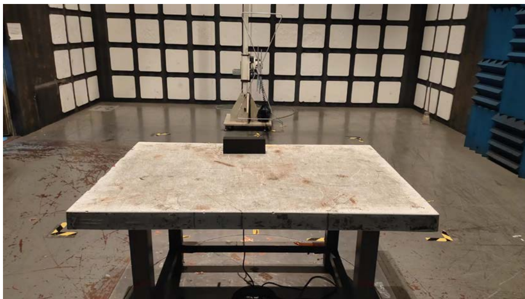
FRONT VIEW OF RADIATED EMISSION
