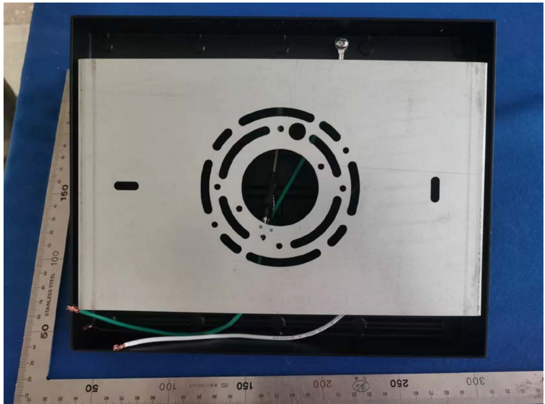
FIGURE 2 LED LUMINAIRE (M/N: OUT-HA-MB) GENERAL BACK
