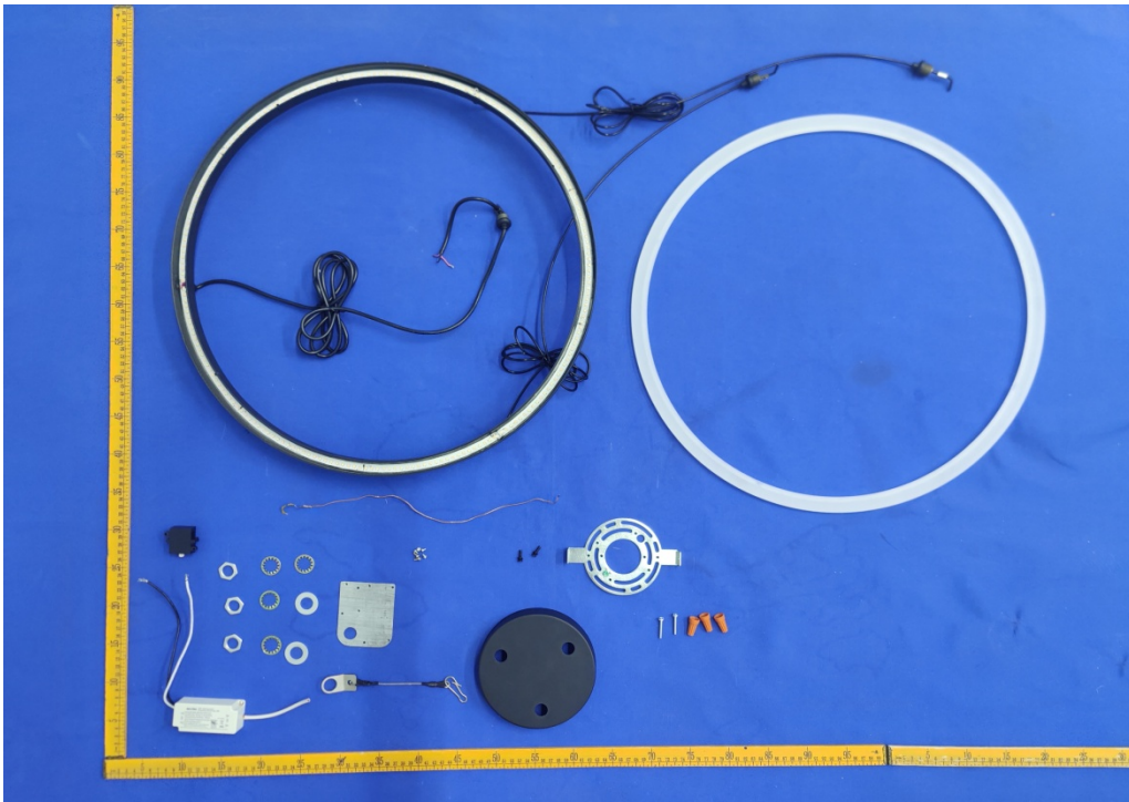
Fig.6(Model: OPDT-NORT)
