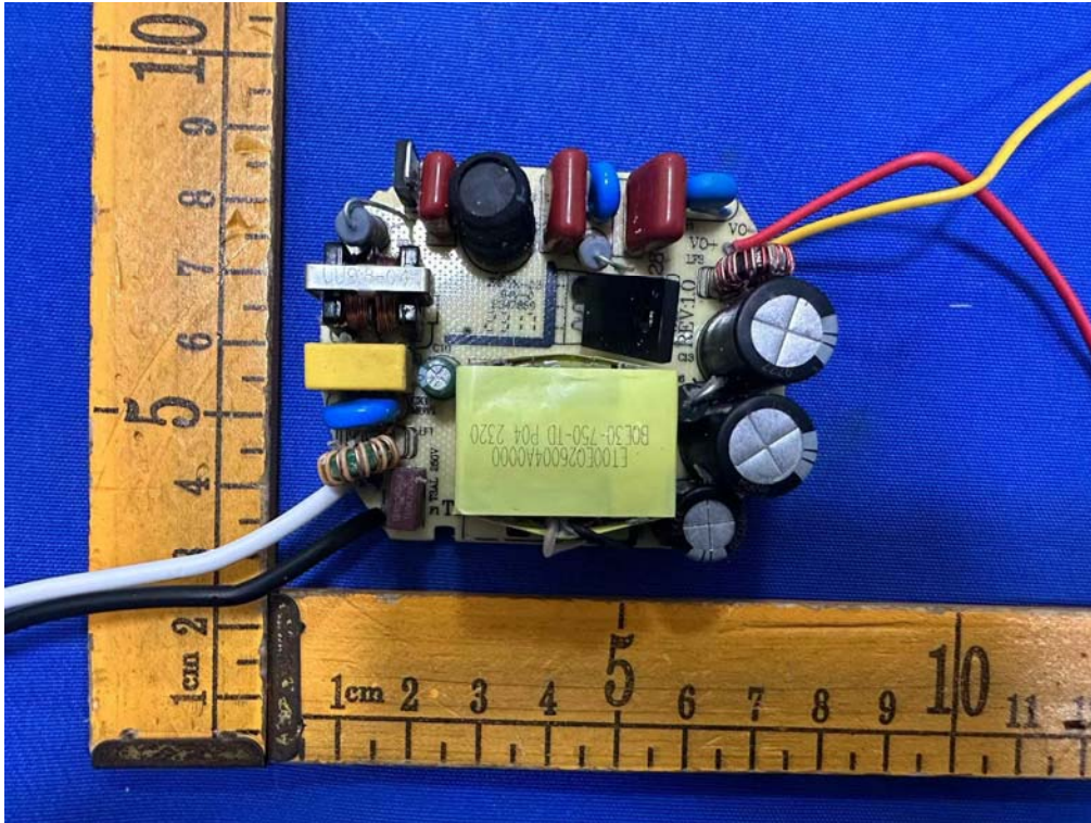
Fig.7(Model: FM-SB )
