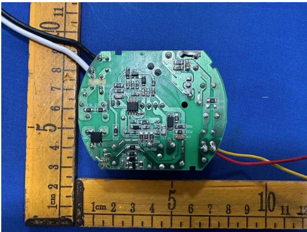
Fig.8(Model: FM-SB )
