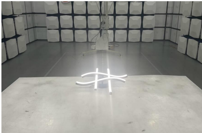
Radiated Disturbance below 1GHz
