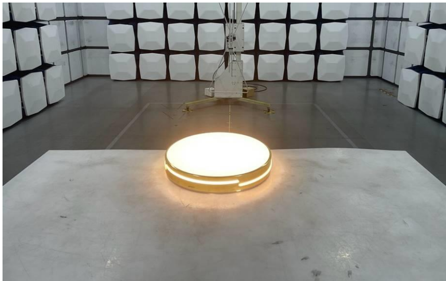
Radiated Disturbance below 1GHz
