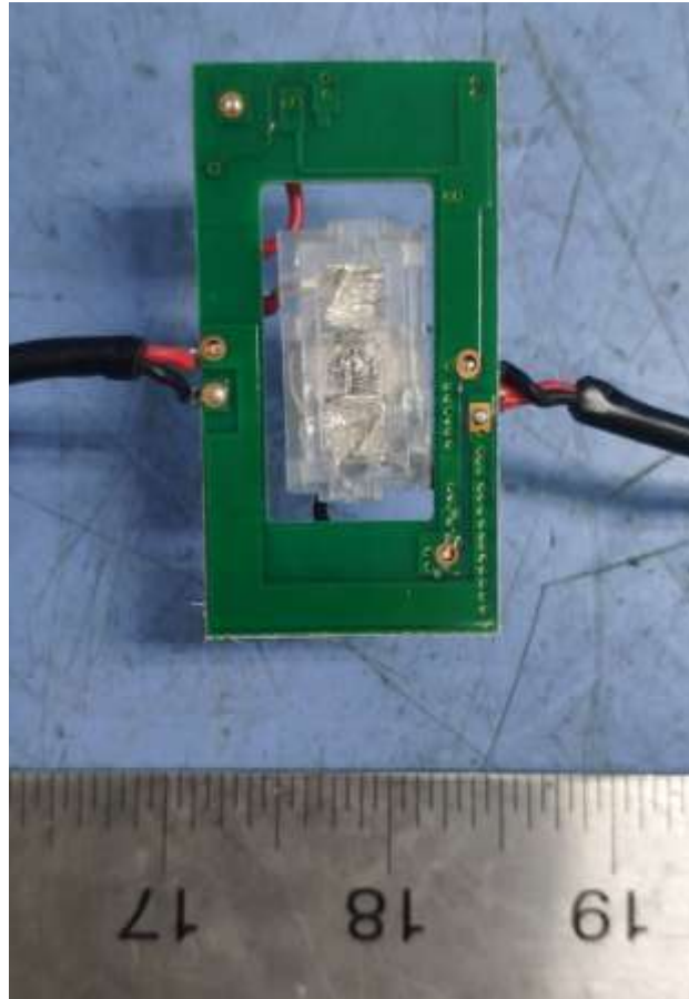
Dimmer PCB View
