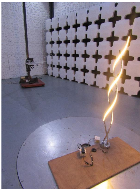
Radiated Emission (30 MHz–1000 MHz)
