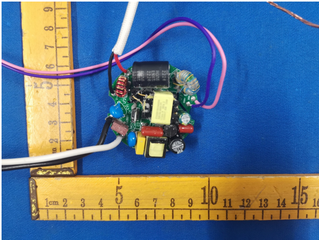
Fig.6(Model: 6OUT-DS )
