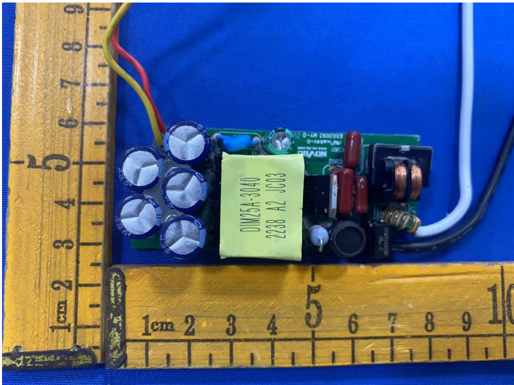
Fig.6 (Model:48PDT-DEC)
