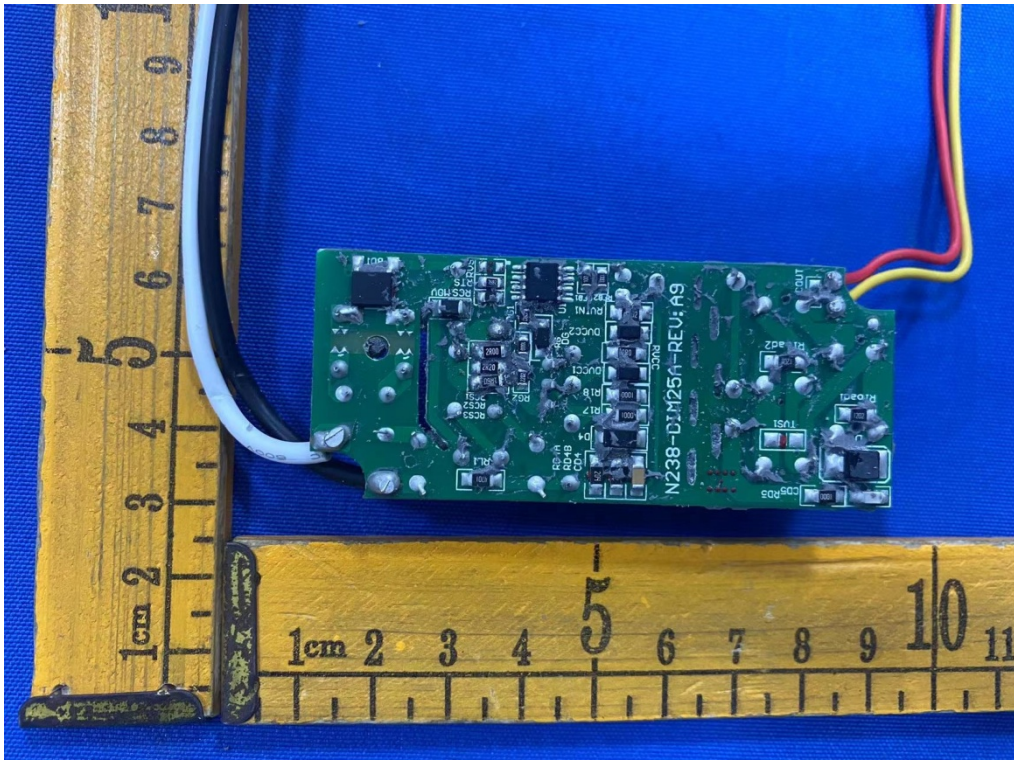
Fig.5 (Model:48PDT-DEC)
