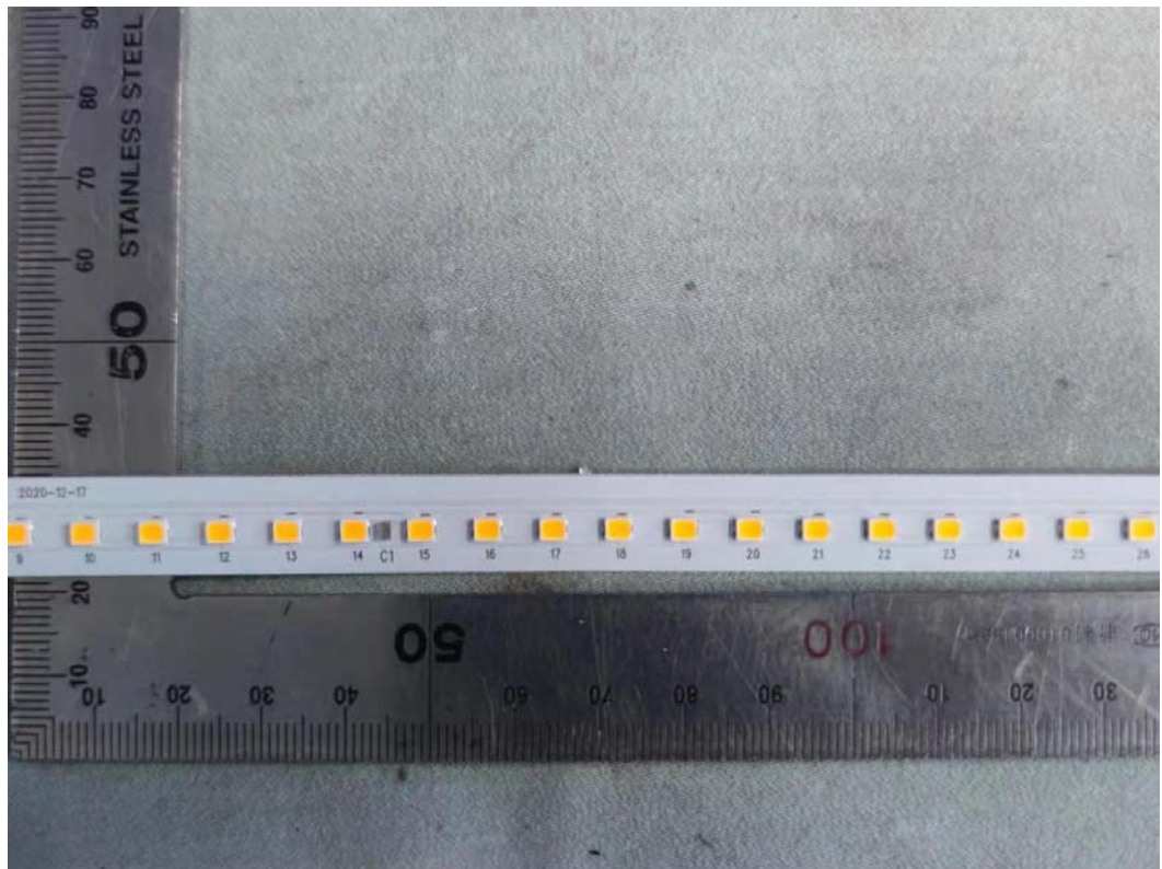
FIGURE 5 LED PANEL (M/N: 15FLPR-SP3-WH) LED FRONT VIEW
