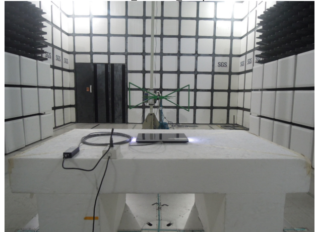
NFC_Radiated_Setup
