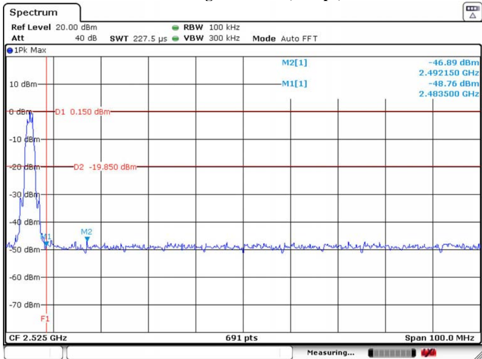
GFSK High Channel (2Mbps)
