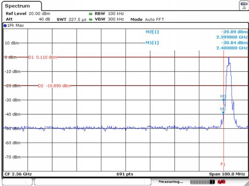
GFSK Low Channel (2Mbps)
