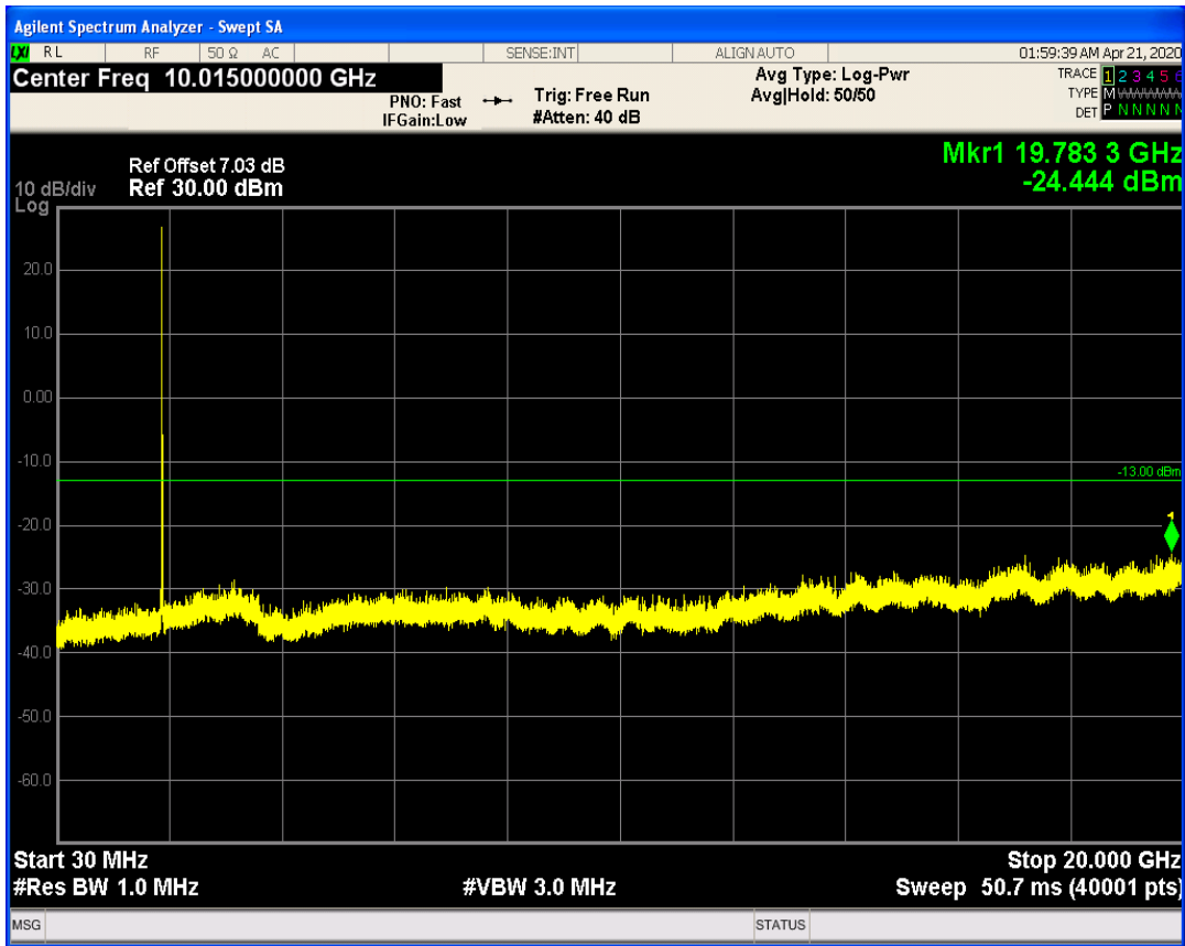
LTE Band25 QAM16 BW=1.4MHz Channel=26047 RB Size=6 Position=#0
