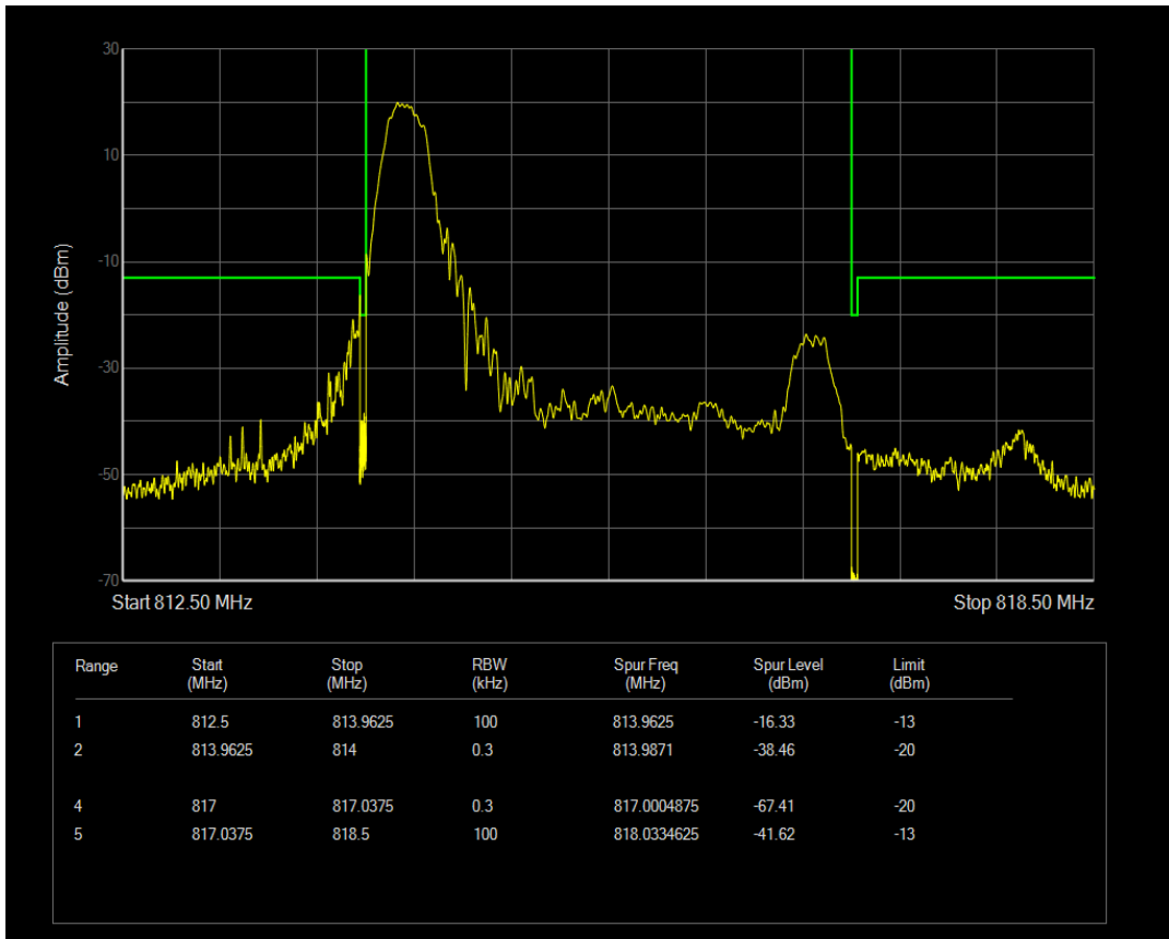
LTE Band26 QAM16 BW=3MHz Channel=26705 RB Size=1 Position=#Max
