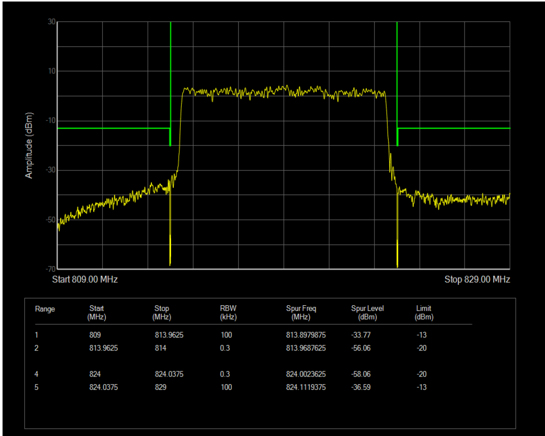
LTE Band26 QAM16 BW=10MHz Channel=26740 RB Size=50 Position=#0
