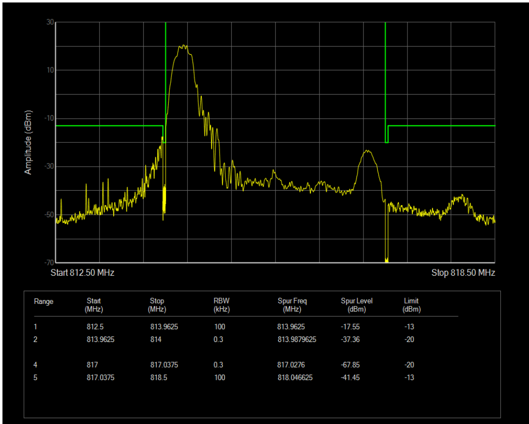
LTE Band26 QPSK BW=3MHz Channel=26705 RB Size=1 Position=#0
