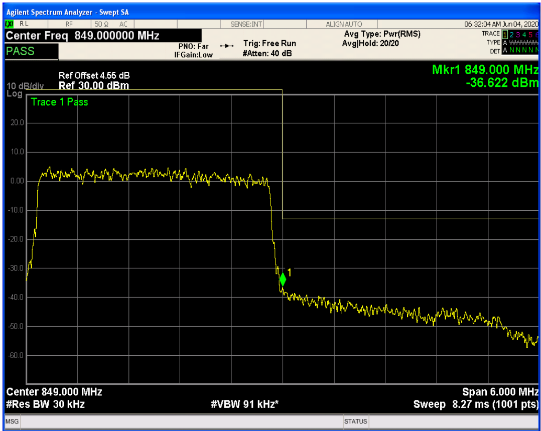
LTE Band26 QAM16 BW=3MHz Channel=27025 RB Size=1 Position=#0
