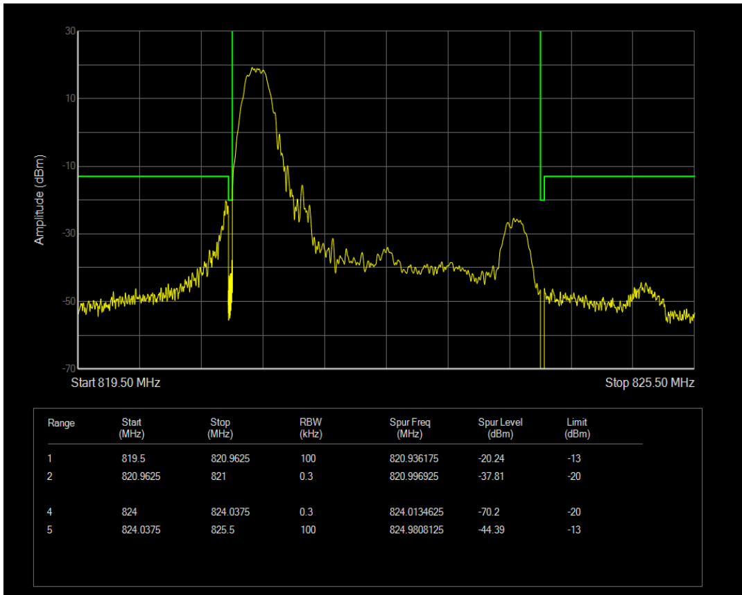
LTE Band26 QAM16 BW=3MHz Channel=26775 RB Size=1 Position=#0
