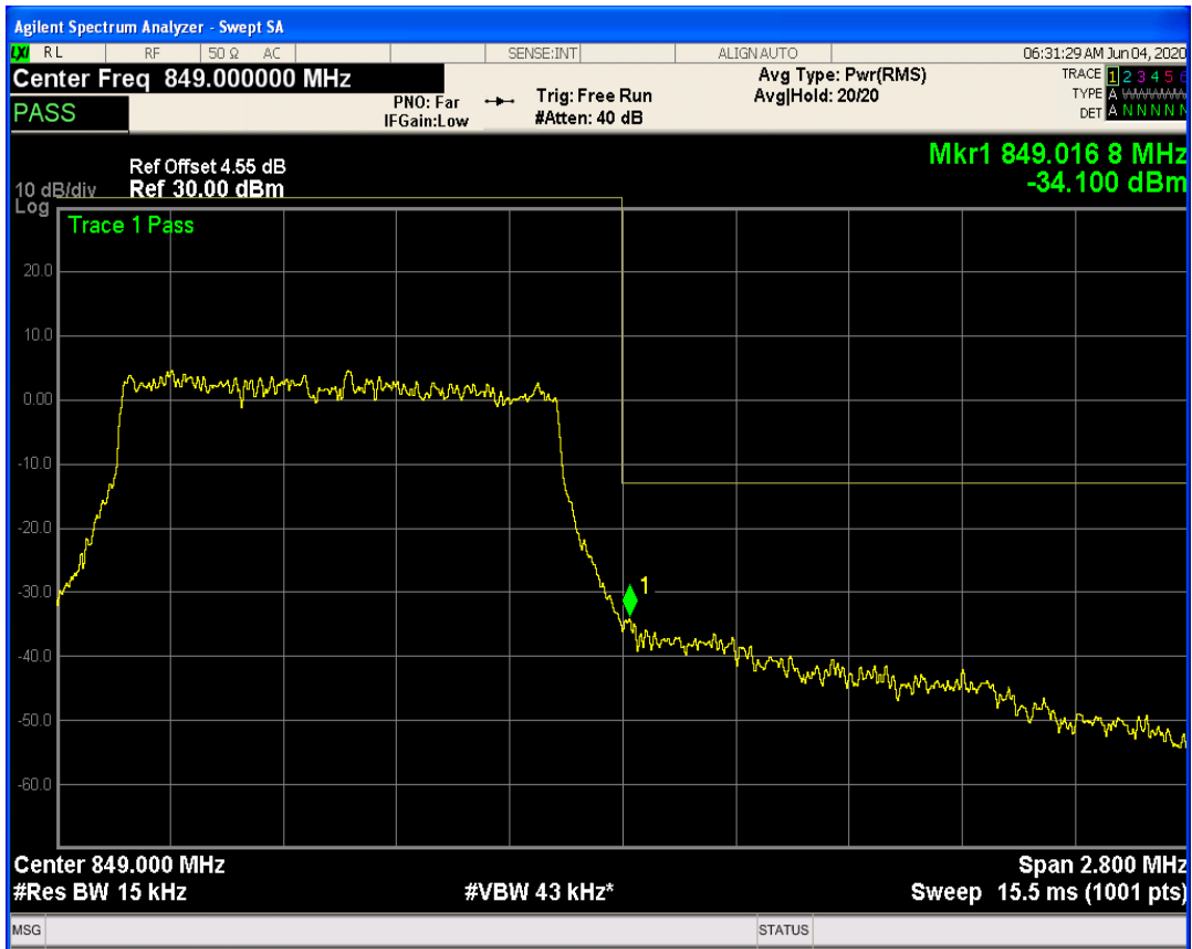
LTE Band26 QAM16 BW=1.4MHz Channel=27033 RB Size=6 Position=#0
