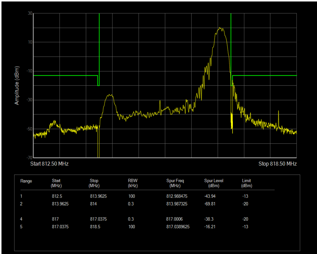
LTE Band26 QPSK BW=3MHz Channel=26705 RB Size=1 Position=#Max
