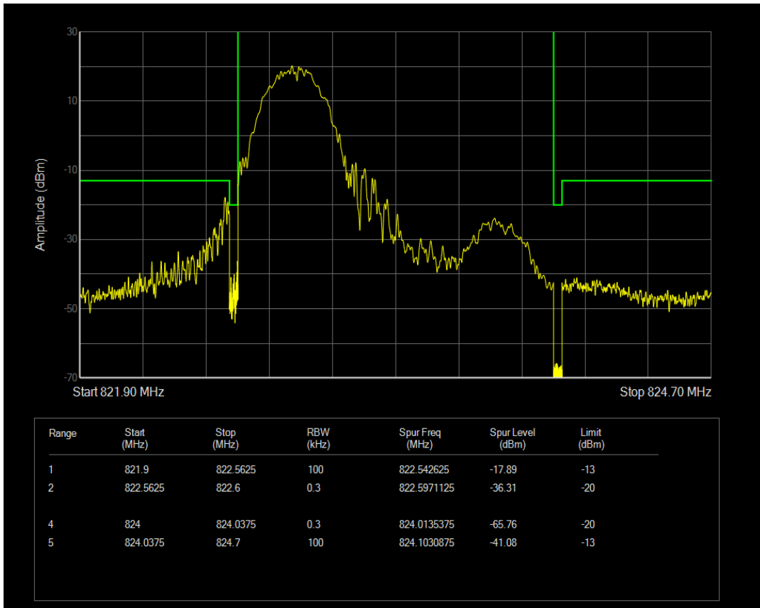
LTE Band26 QAM16 BW=1.4MHz Channel=26783 RB Size=1 Position=#0
