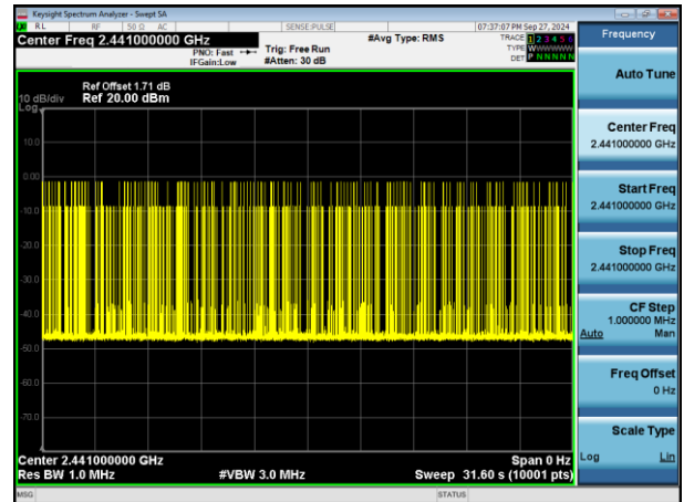
Accumulate(DH3)
