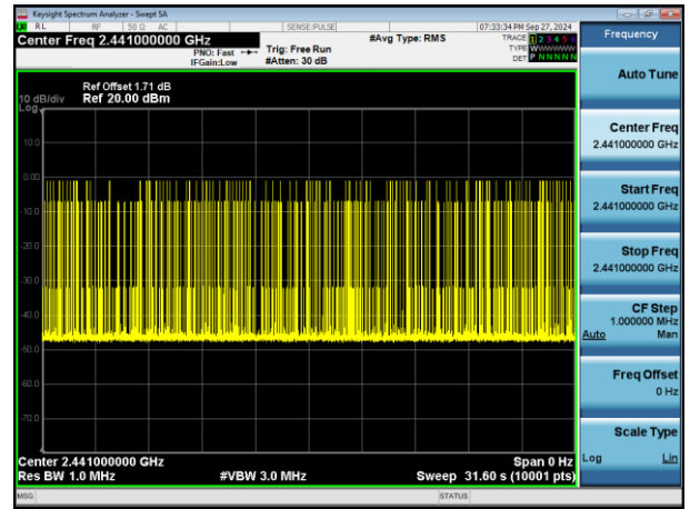
Accumulate(2DH5)
