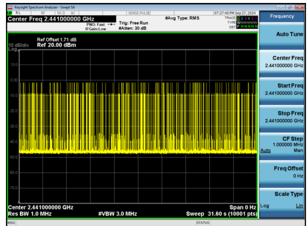
Accumulate(DH5)
