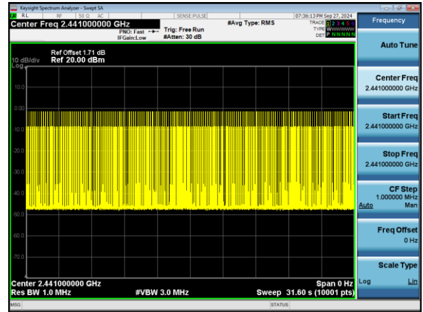
Accumulate(DH1)
