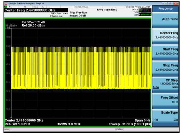
Accumulate(2DH1)
