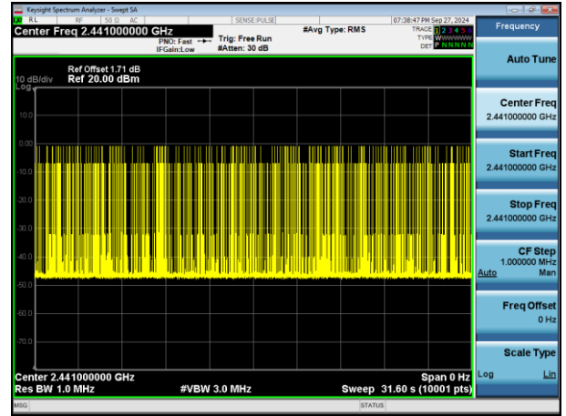
Accumulate(2DH3)
