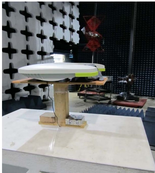
Radiated emissions test setup with Horn antenna.
