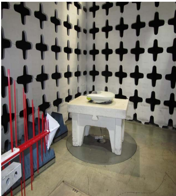
Radiated emissions test setup with Biconilog antenna.
