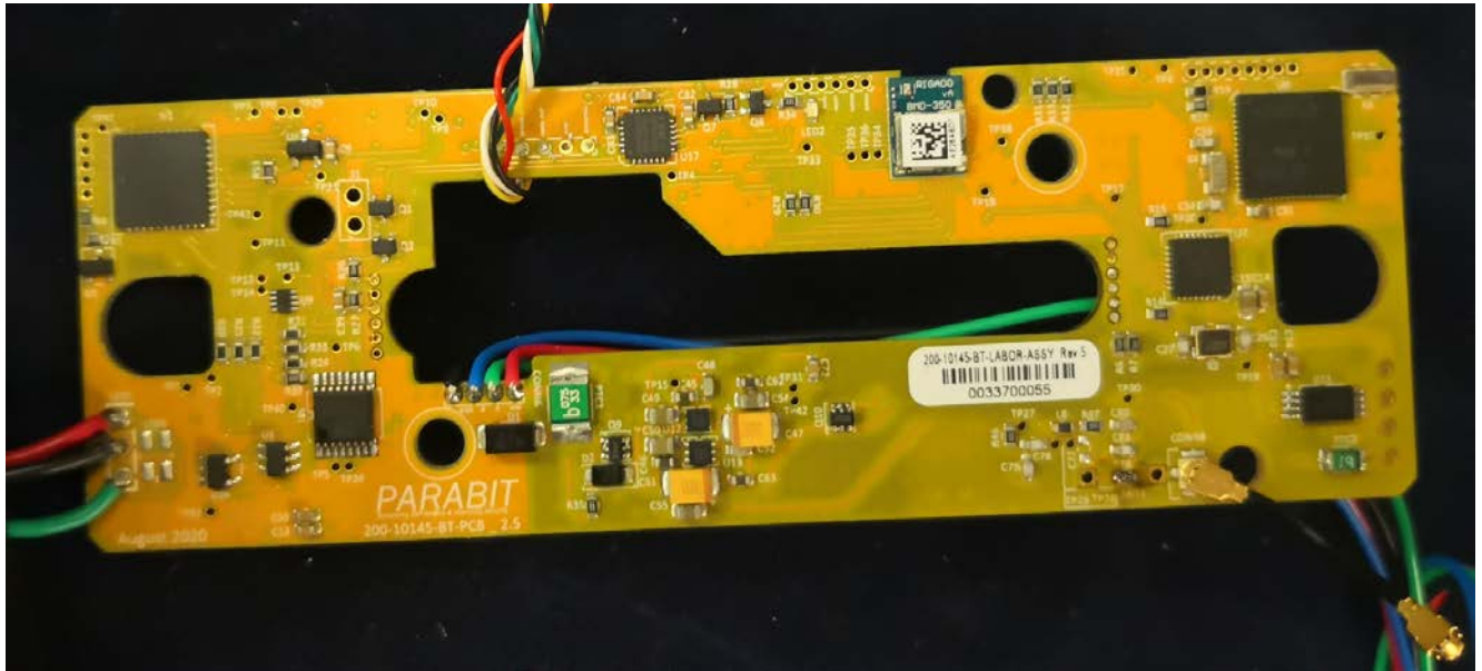
Figure 9.7 PCB Front Side View
