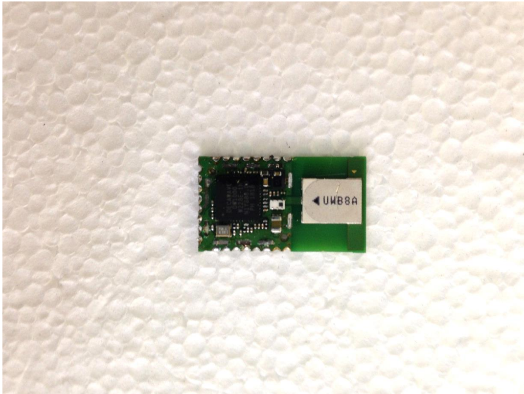
Figure 1. UWB Radio Module, Shield Removed
