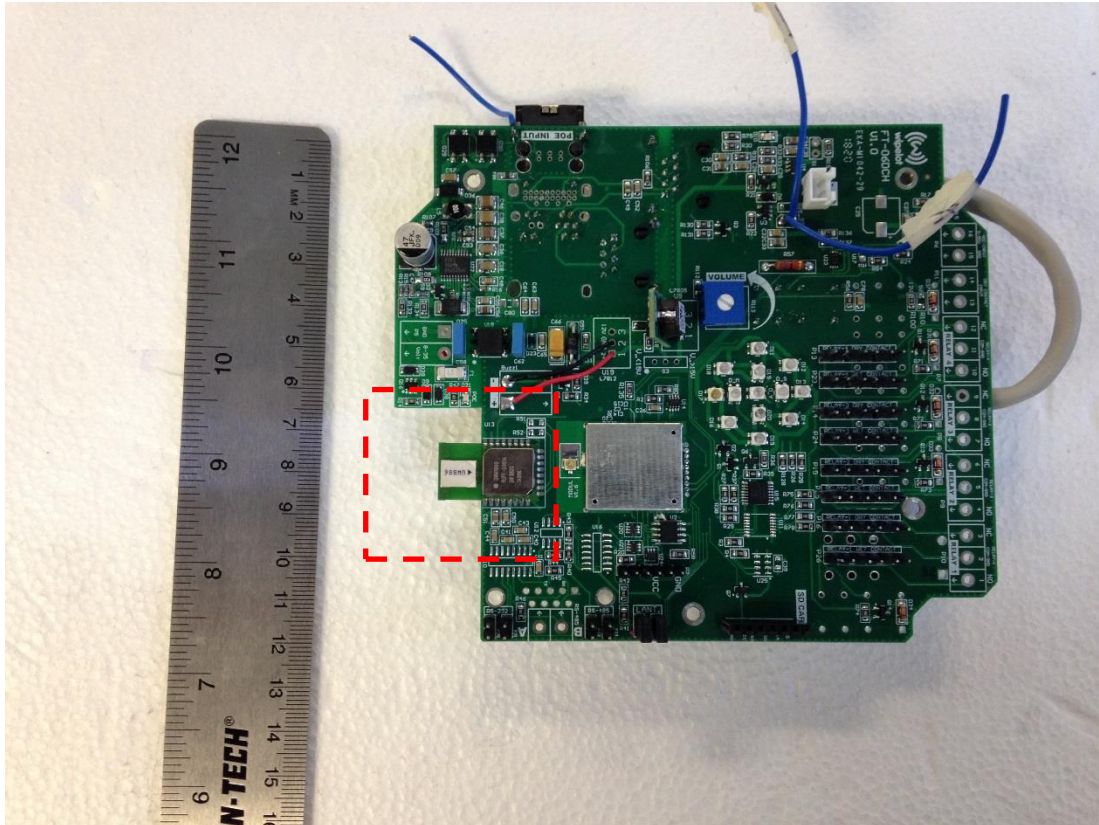
Figure 1. UWB Radio Module on Evaluation Board
