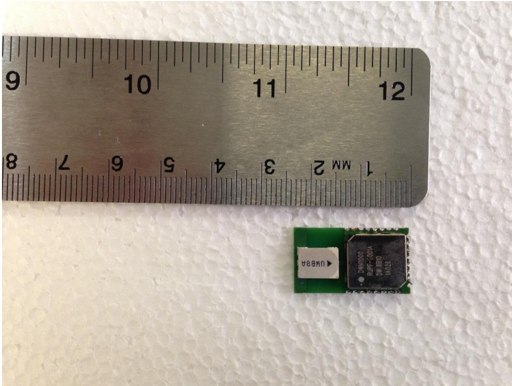
Figure 2. UWB Radio Module Top View
