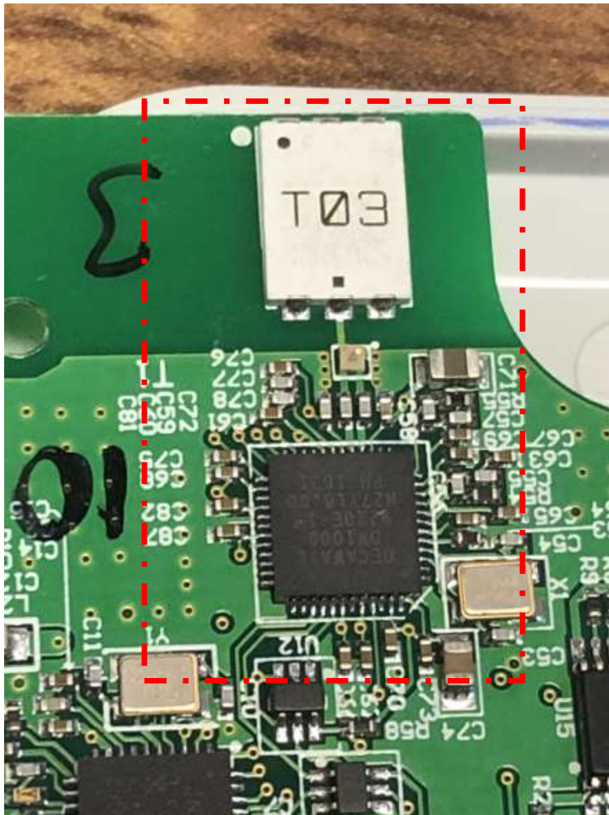
Figure 5. UWB Radio Module Circuit
