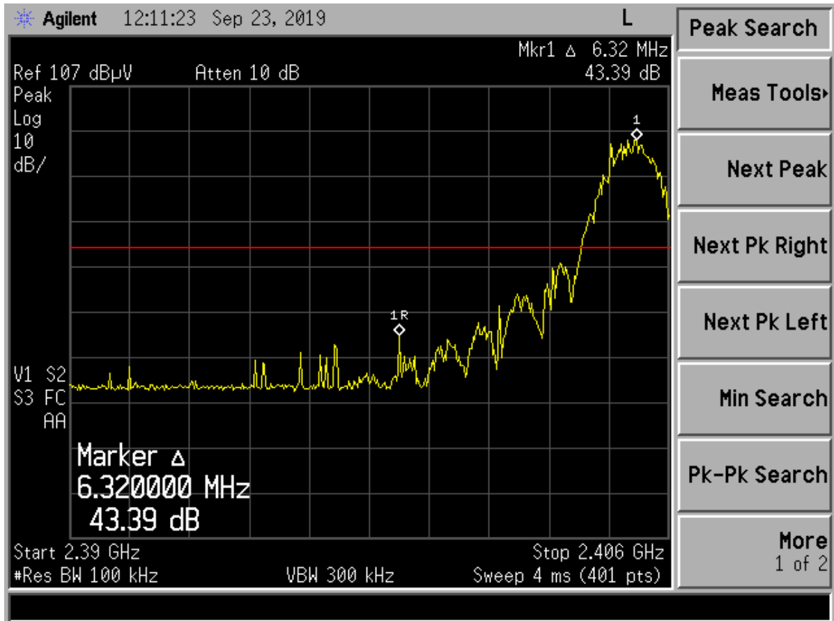
Figure 2. Band Edge Compliance – Low Channel Delta
