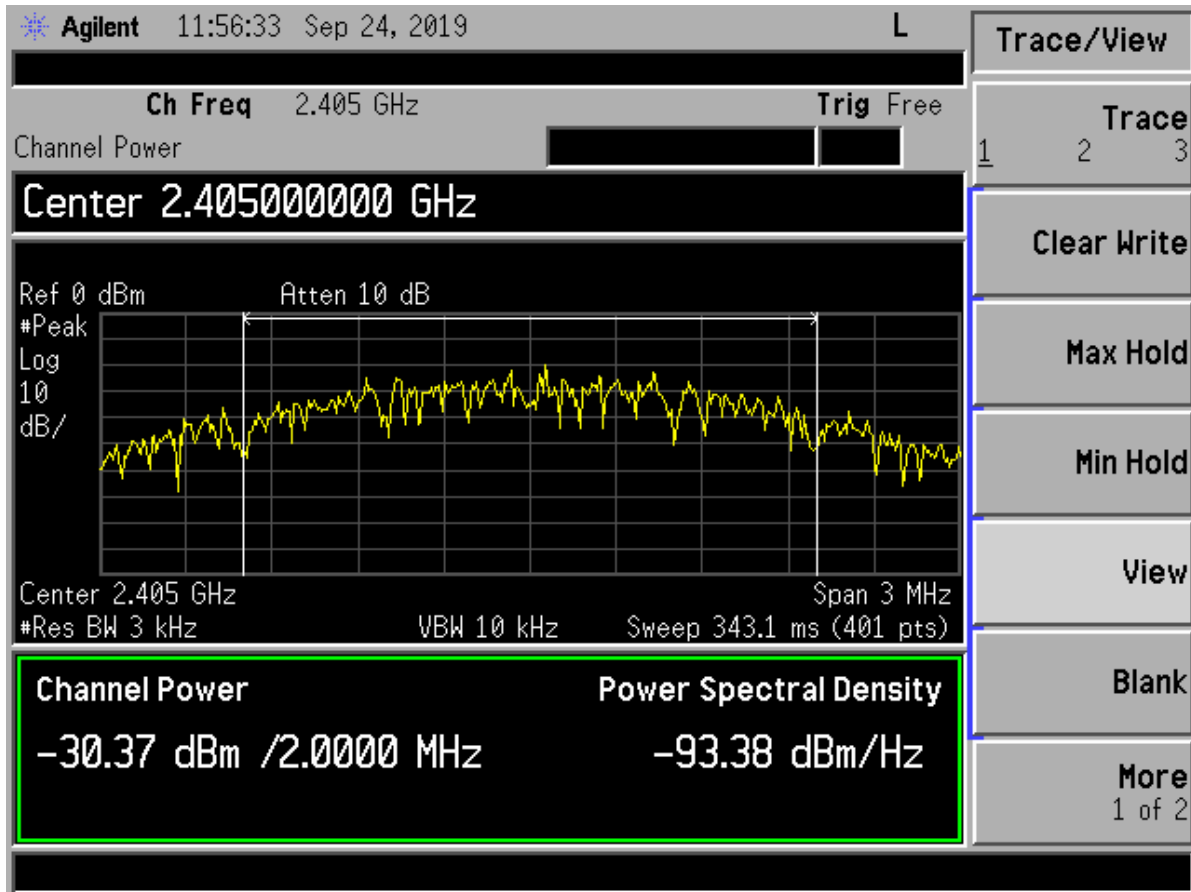
Figure 9. Peak Antenna Conducted Output Power, Low Channel
