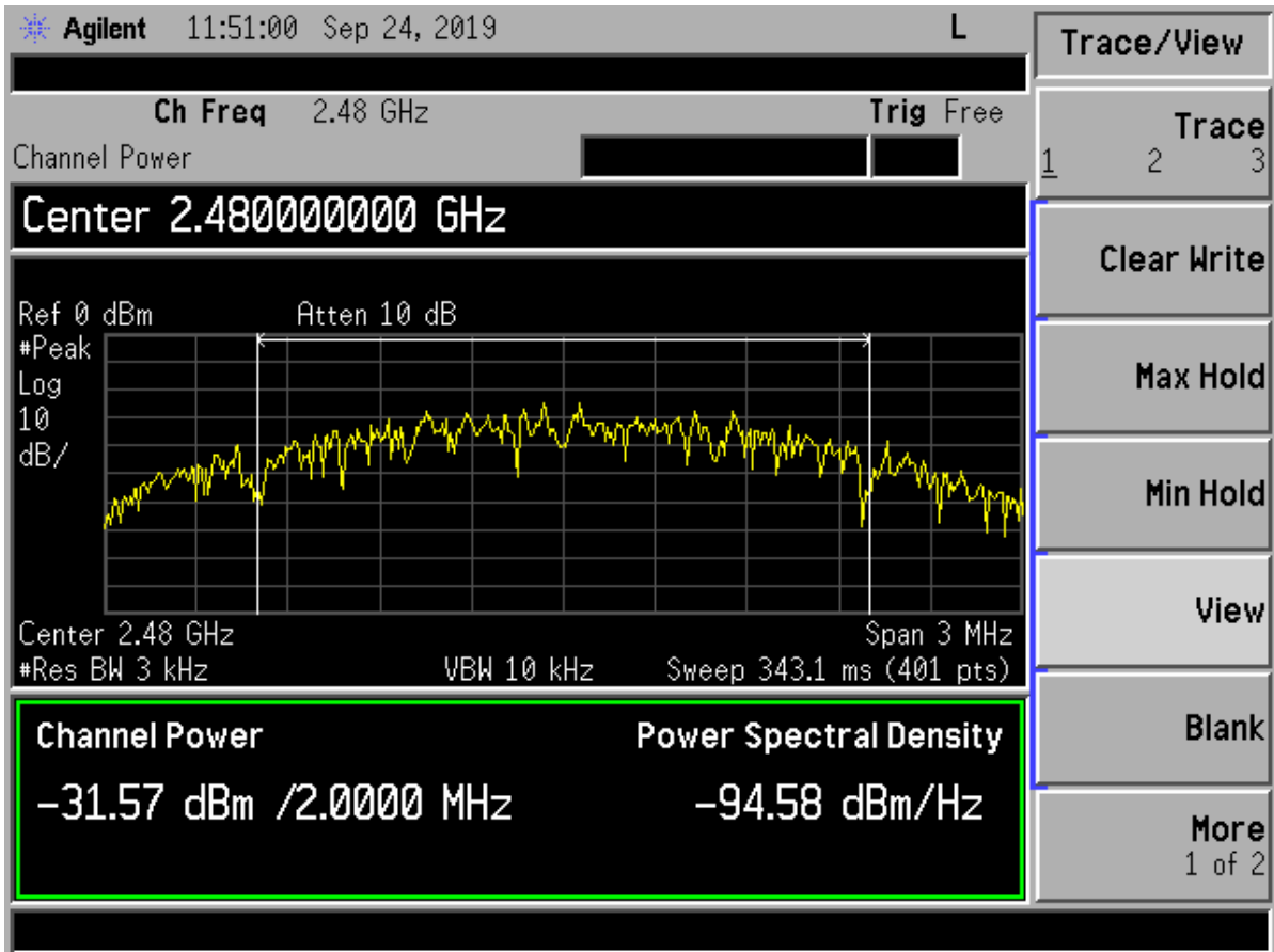
Figure 11. Peak Antenna Conducted Output Power, High Channel
