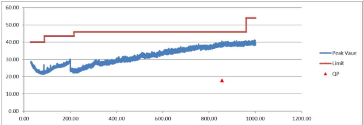
Figure 12. Radiated Emissions Graphical Data, TX, 30-1000 MHz - Horizontal
