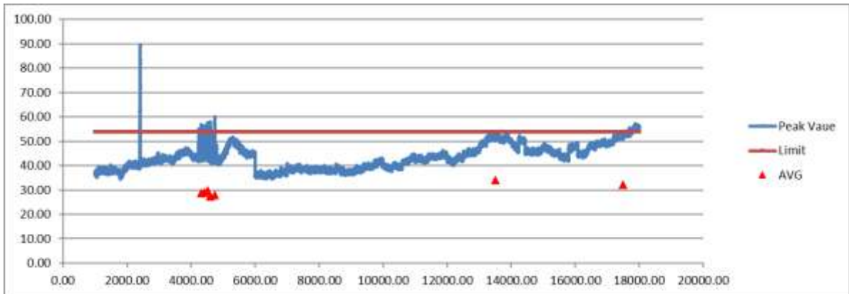
Figure 15. Radiated Emissions Graphical Data, TX, 1 -18GHz – Vertical
