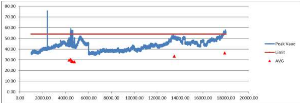
Figure 14. Radiated Emissions Graphical Data, TX, 1 -18GHz - Horizontal
