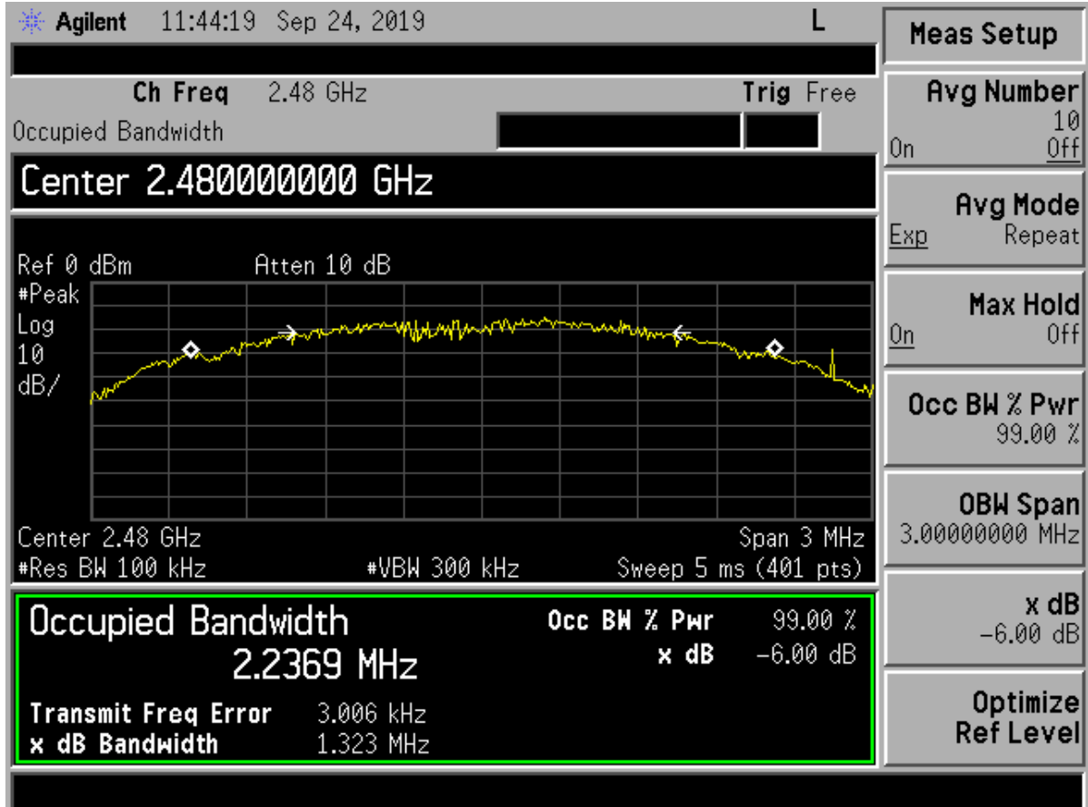
Figure 8. 6 dB Bandwidth High Channel
