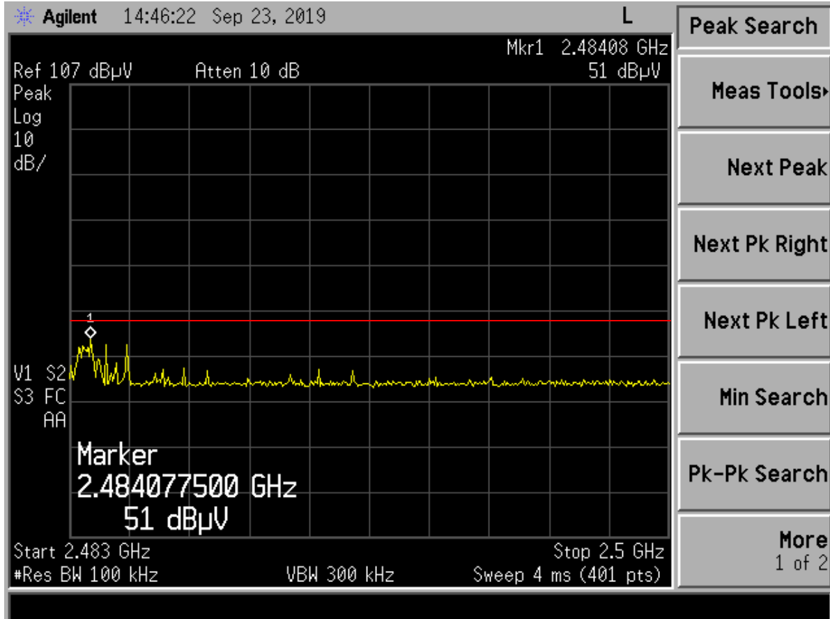
Figure 5. High Channel Restricted Band – Peak
