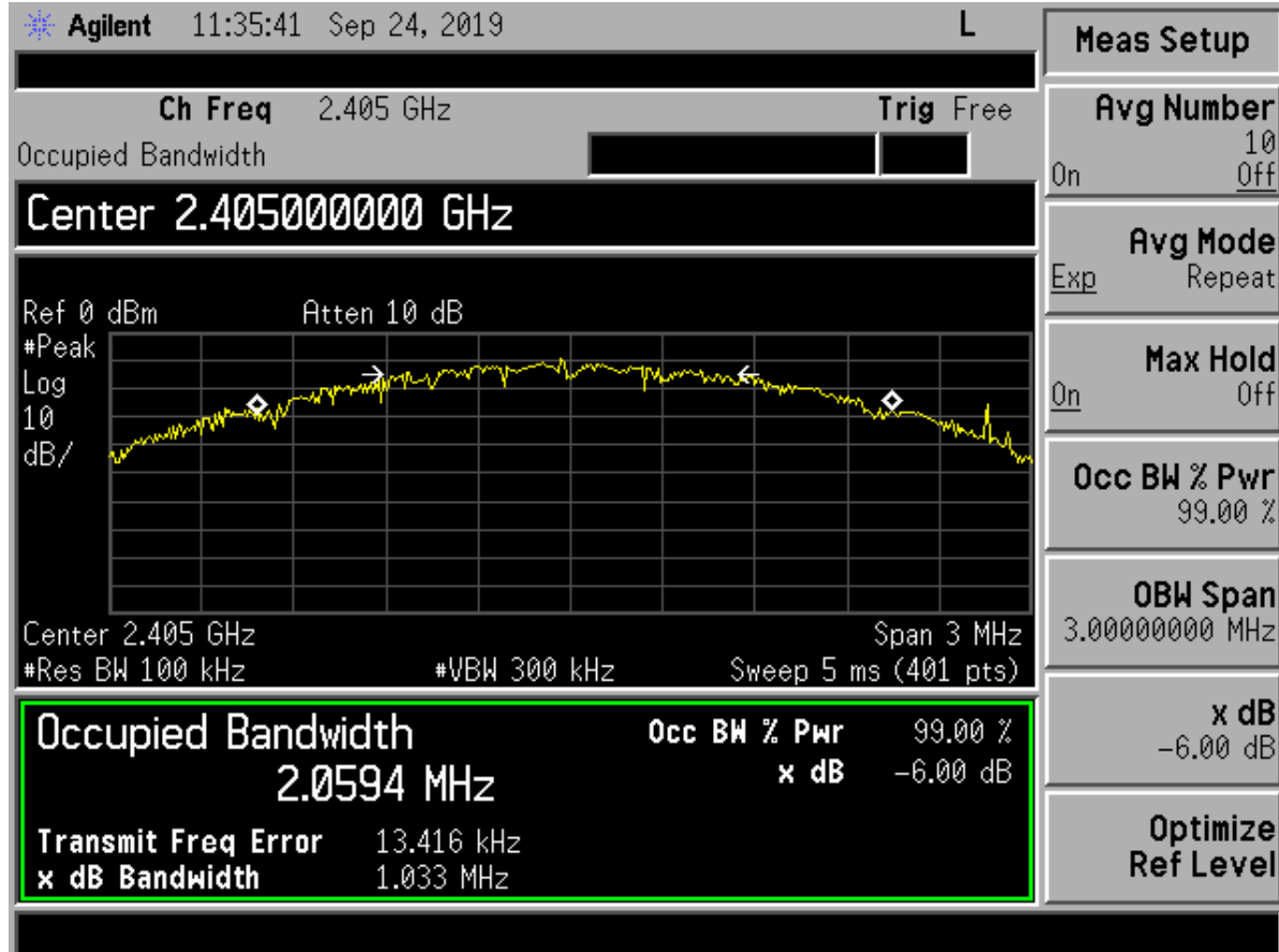
Figure 6. 6 dB Bandwidth Low Channel
