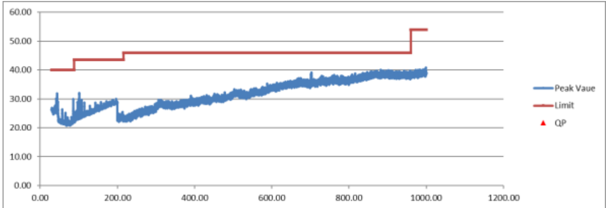
Figure 13. Radiated Emissions Graphical Data, TX, 30-1000 MHz – Vertical
