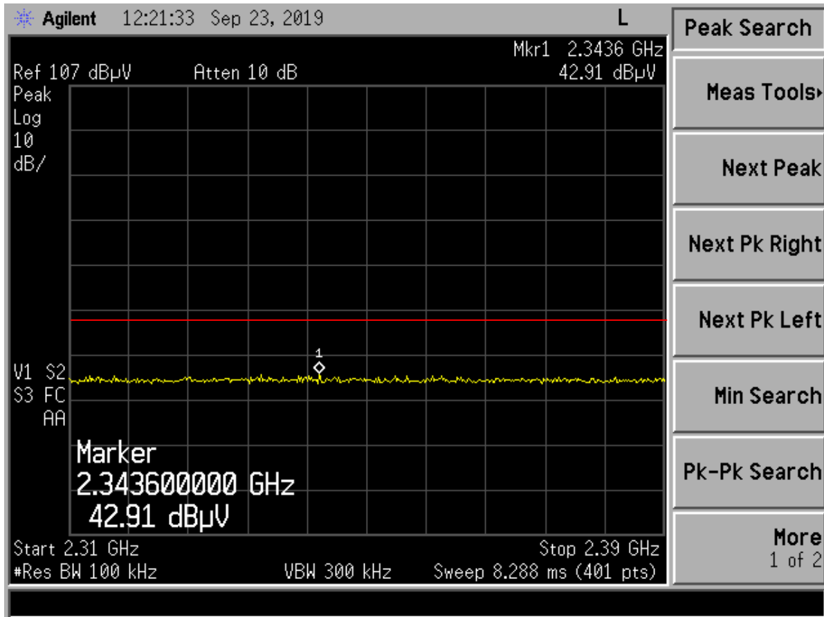
Figure 3. Low Channel Restricted Band – Peak
