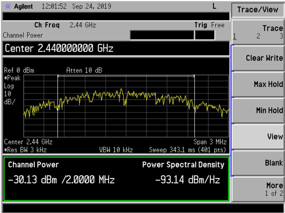
Figure 10. Peak Antenna Conducted Output Power, Mid Channel
