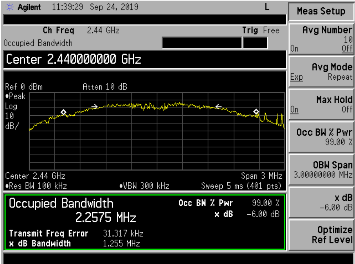
Figure 7. 6 dB Bandwidth Mid Channel
