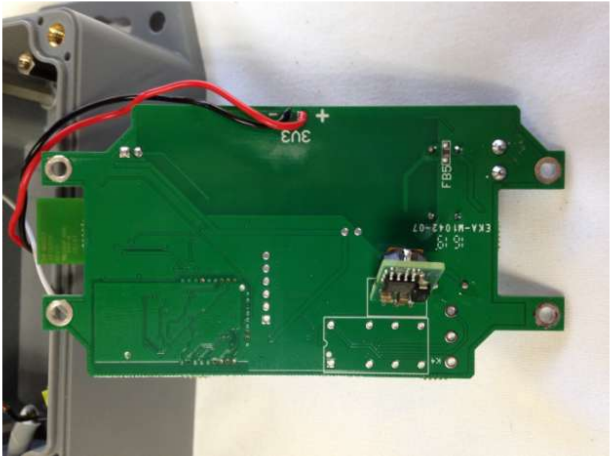
Figure 3. Main PCB Back Side
