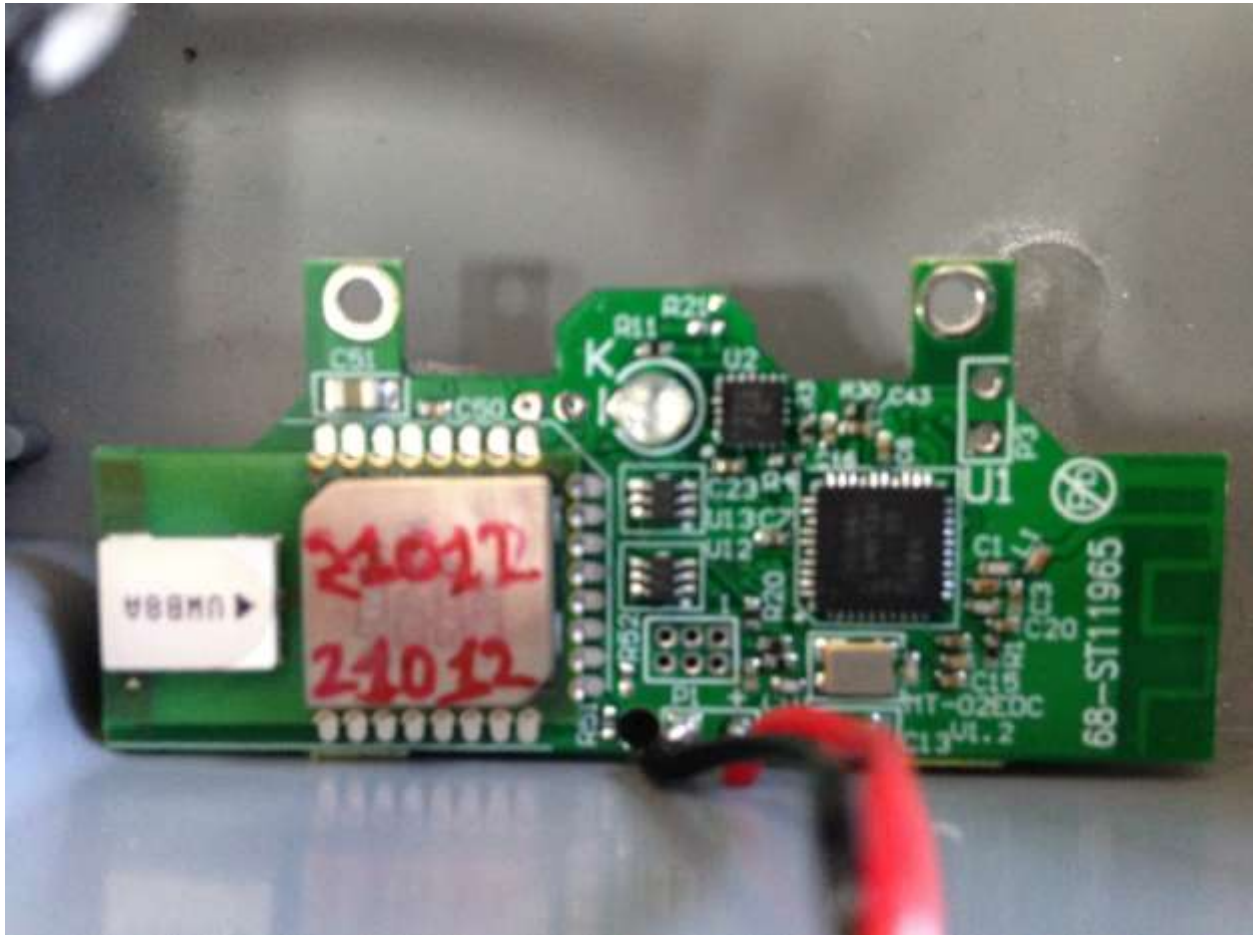
Figure 4. Secondary PCB with UWB Radio #2 and Disabled 2.4 GHz radio
