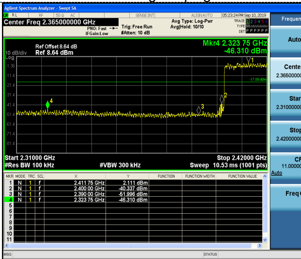
Left Band edge hopping on
