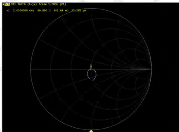
Impedance Test-Body
