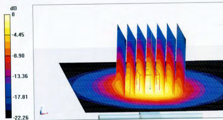
0 dB = 19.7 W/kg = 12.94 dBW/kg
