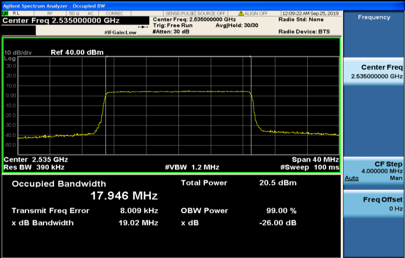
Band7-20MHz-16QAM-21350-100RB#0-17.946
