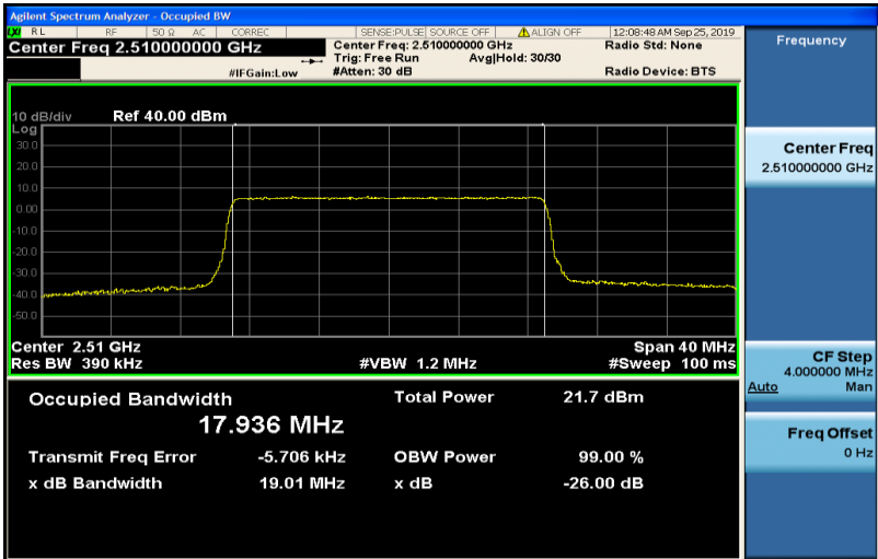
Band7-20MHz-QPSK-21100-100RB#0-17.936
