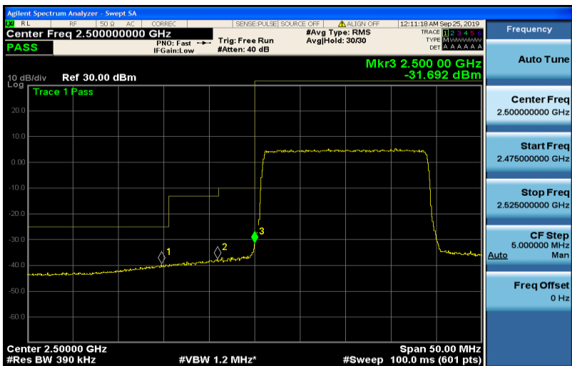
Band7-20MHz-16QAM-21350-1RB#0
