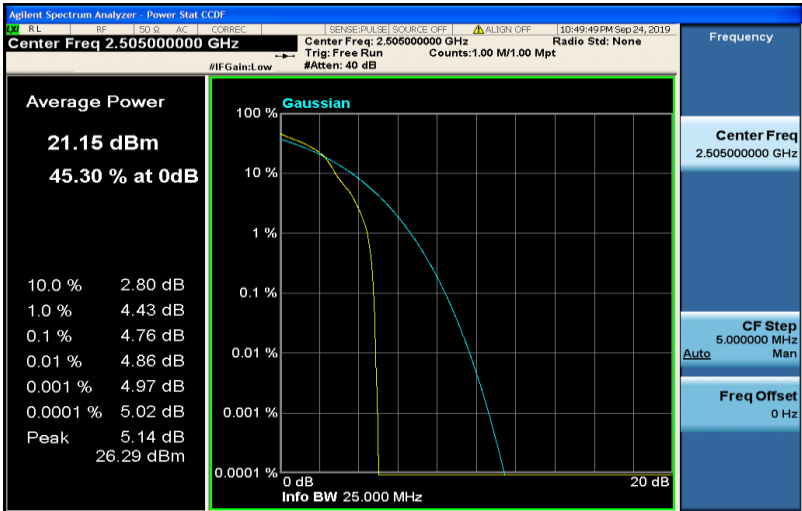
Band7-10MHz-16QAM-20800-50RB#0
