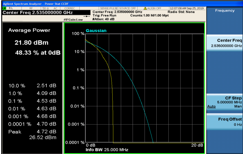
Band7-15MHz-QPSK-21100-75RB#0
