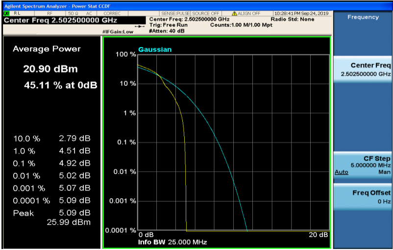
Band7-5MHz-16QAM-20775-25RB#0
