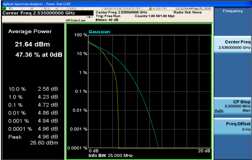
Band7-20MHz-QPSK-21100-100RB#0
