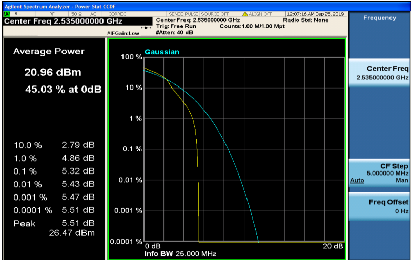
Band7-15MHz-16QAM-21100-75RB#0
