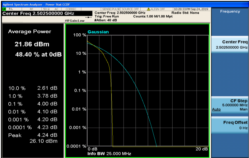
Band7-5MHz-QPSK-20775-25RB#0
