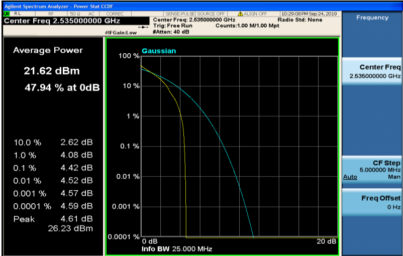
Band7-5MHz-QPSK-21100-25RB#0
