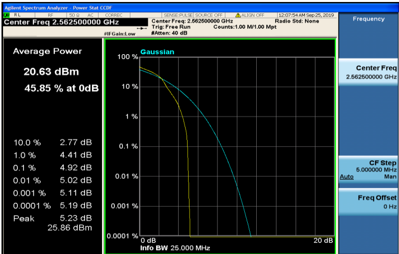
Band7-15MHz-16QAM-21375-75RB#0
