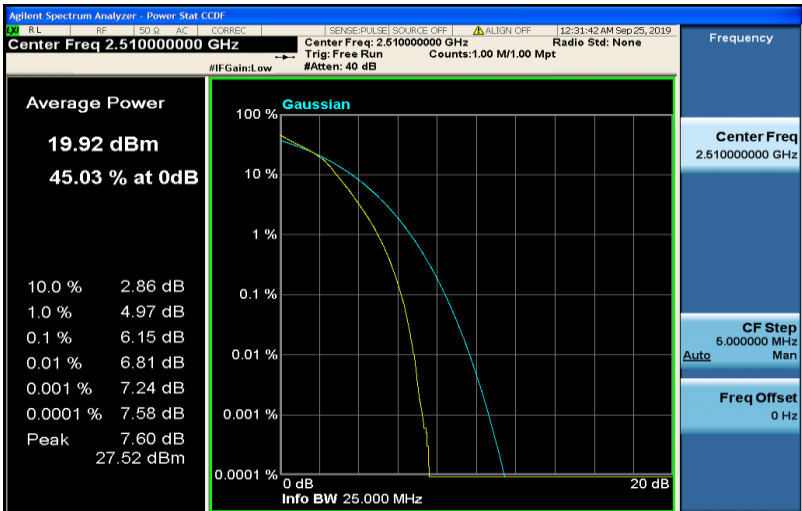
Band7-20MHz-16QAM-21100-1RB#0
