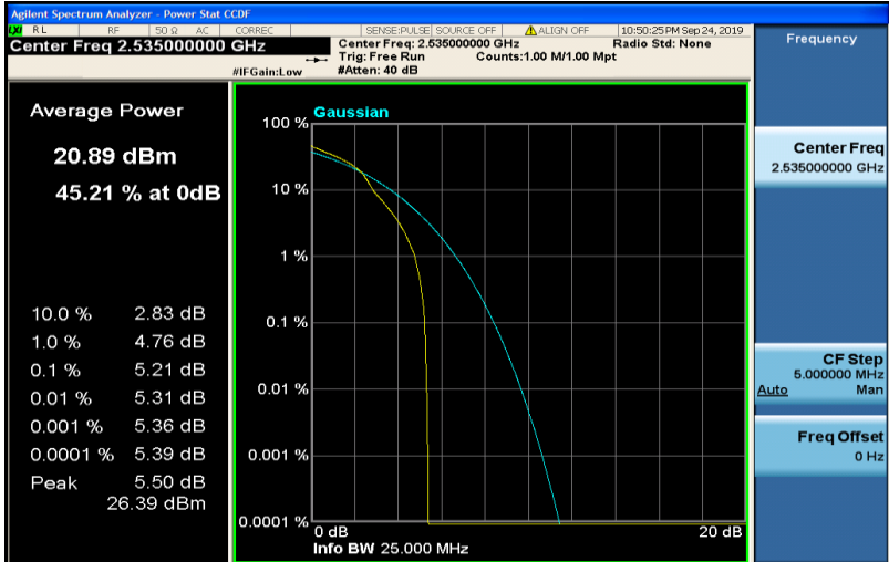
Band7-10MHz-16QAM-21100-50RB#0
