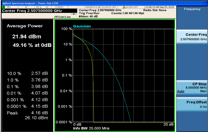
Band7-15MHz-QPSK-20825-75RB#0
