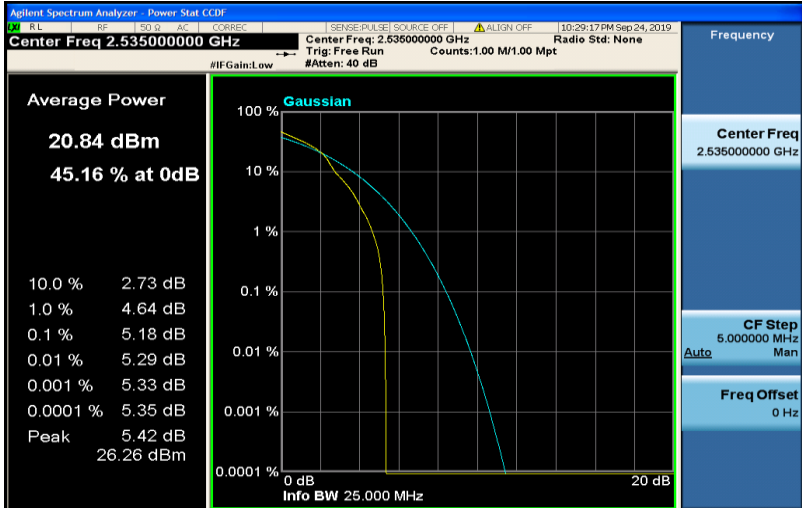
Band7-5MHz-16QAM-21100-25RB#0
