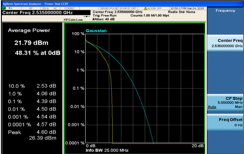
Band7-10MHz-QPSK-21100-50RB#0
