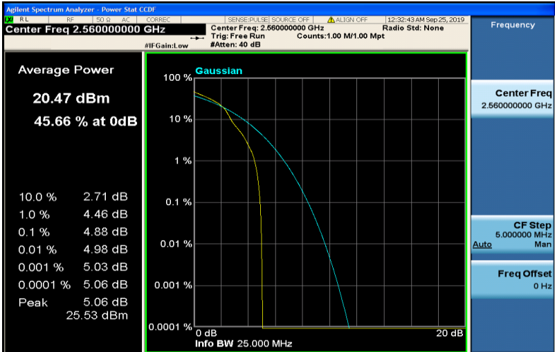
Band7-20MHz-16QAM-21350-100RB#0
