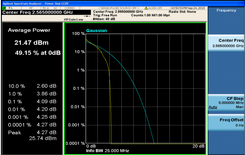
Band7-10MHz-QPSK-21400-50RB#0
