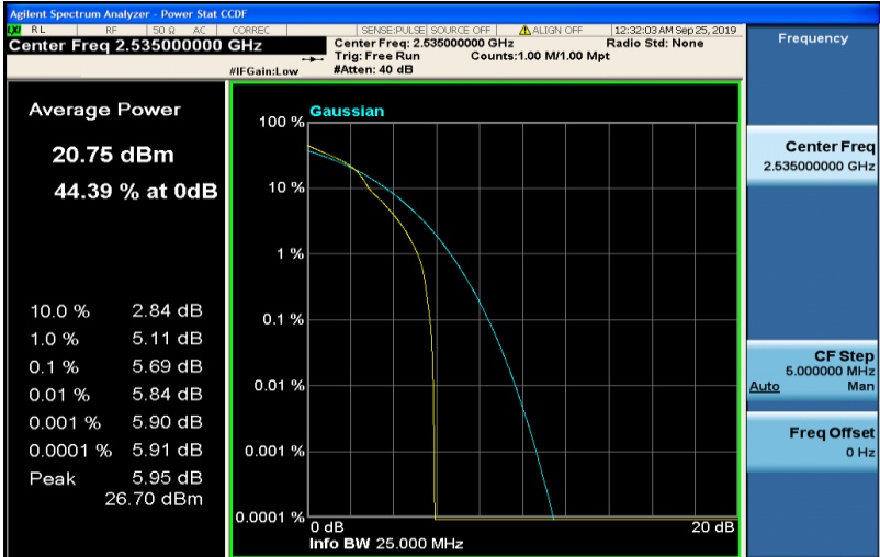
Band7-20MHz-16QAM-21100-100RB#0
