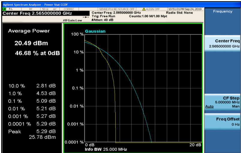
Band7-10MHz-16QAM-21400-50RB#0
