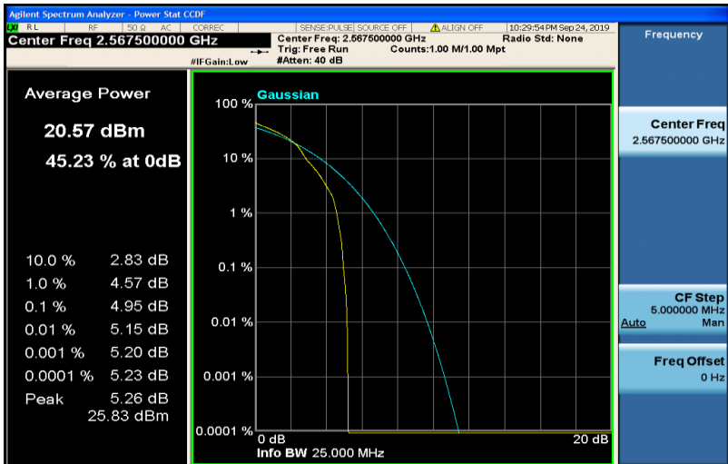
Band7-5MHz-16QAM-21425-25RB#0
