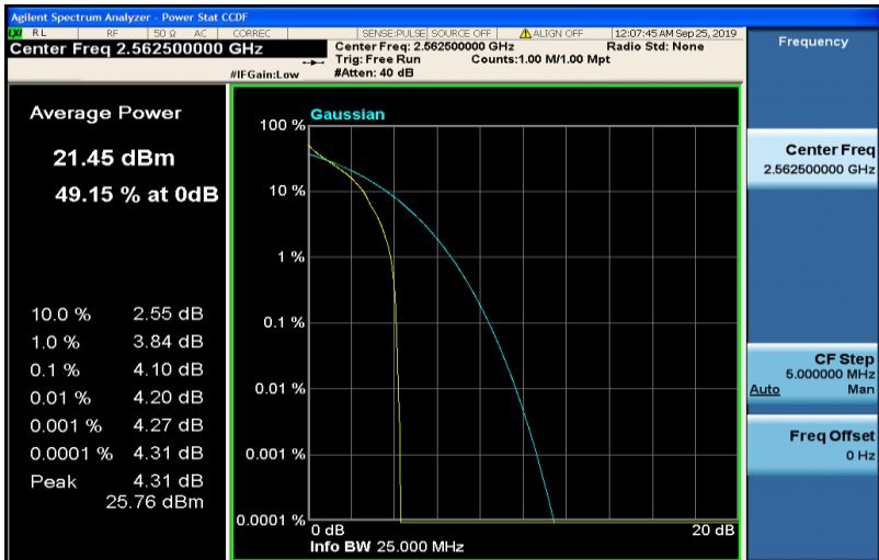
Band7-15MHz-QPSK-21375-75RB#0
