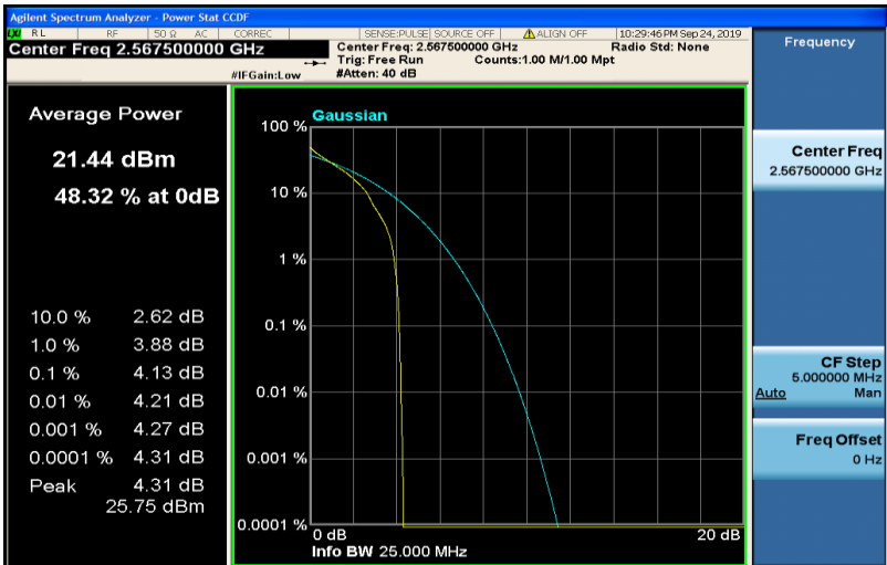
Band7-5MHz-QPSK-21425-25RB#0
