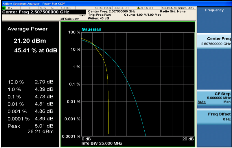
Band7-15MHz-16QAM-20825-75RB#0
