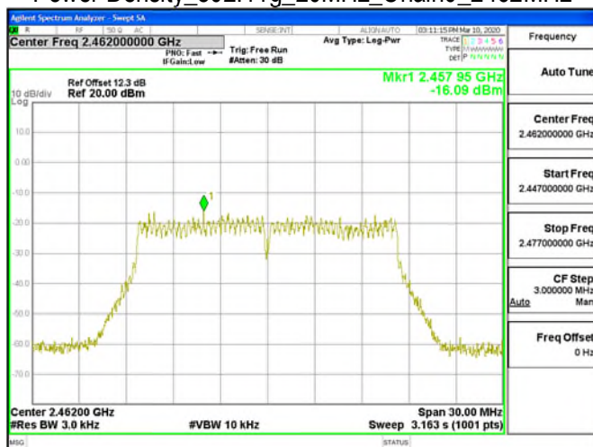
Power Density_802.11g_20MHz_Chain0_2462MHz
