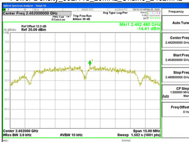
Power Density_802.11b_20MHz_Chain0_2462MHz
