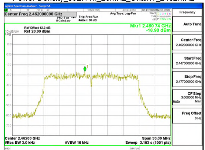
Power Density_802.11n_20MHz_Chain1_2462MHz
