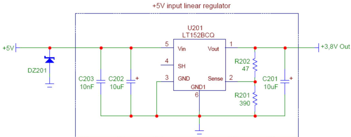
Figure 11: Linear Regulator with 5V Input
