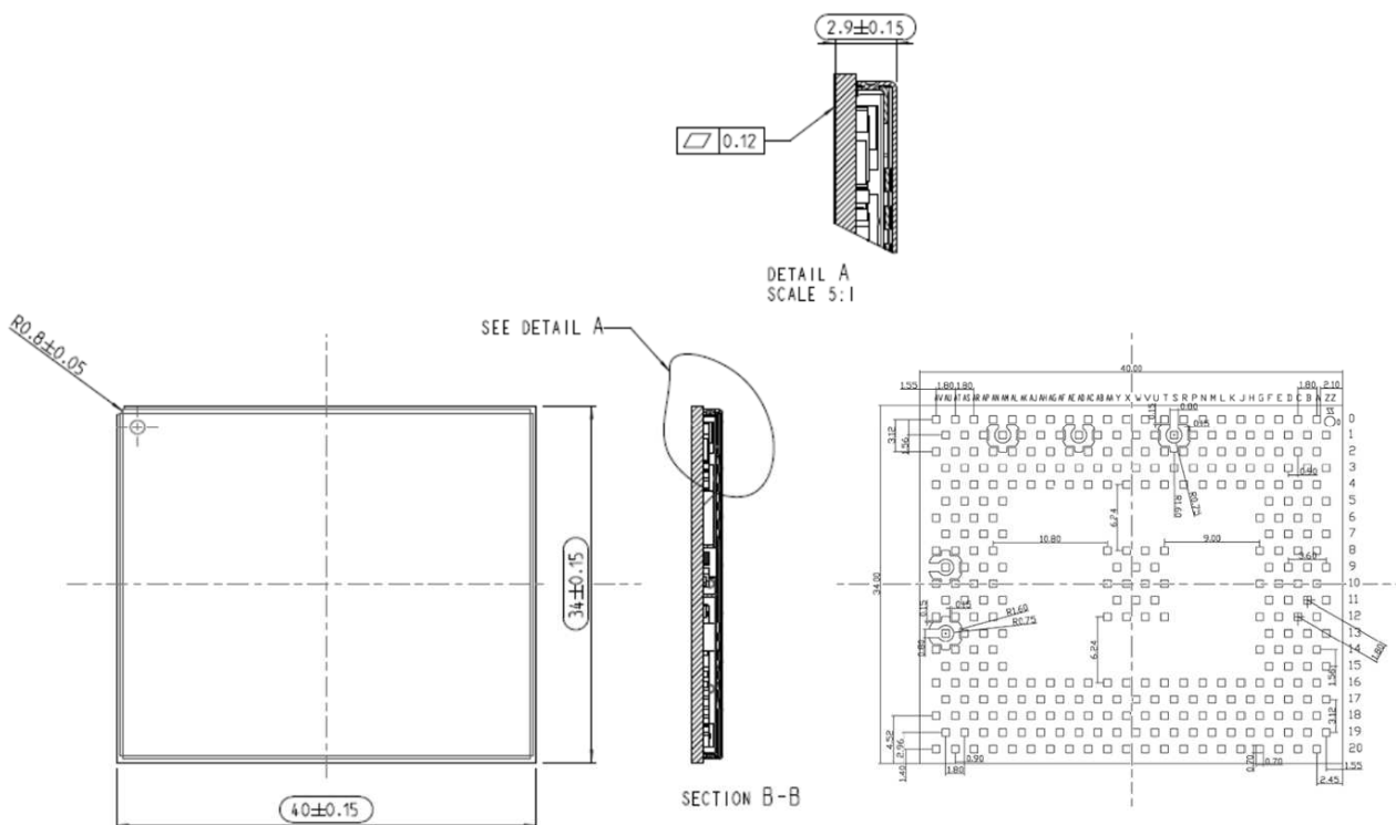
Figure 24: Mechanical Dimensions
