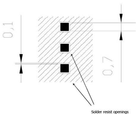
Figure 27: PCB Pad Dimensions
