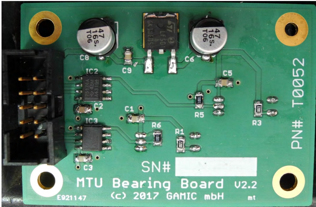
MTU – BEARING – TOP VIEW
