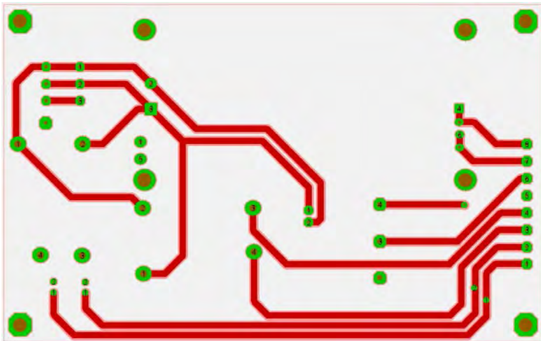
IFD-PSU – BACK VIEW
