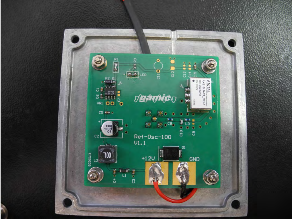
REF-OSC-100 – TOP VIEW
