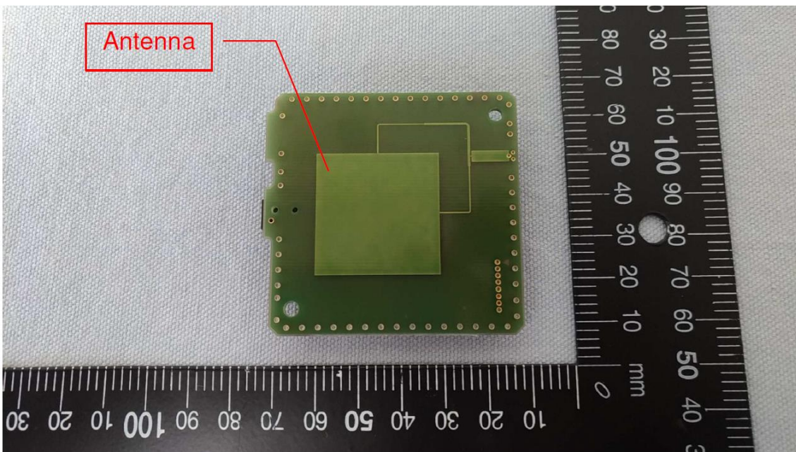
Figure 8 Internal View (Main Board, Back View)
