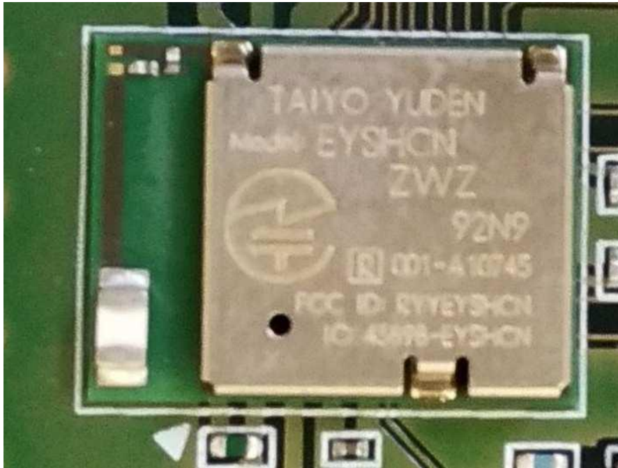
Figure 9 Internal View (BLE Module)
