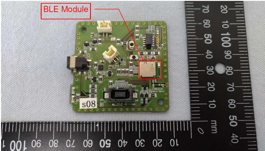
Figure 7 Internal View (Main Board, Front View)
