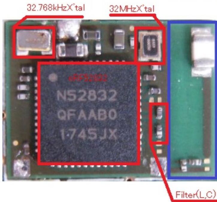
Figure 10 Internal View (BLE Module without shield) *integral antenna(blue-marked) was not used.
