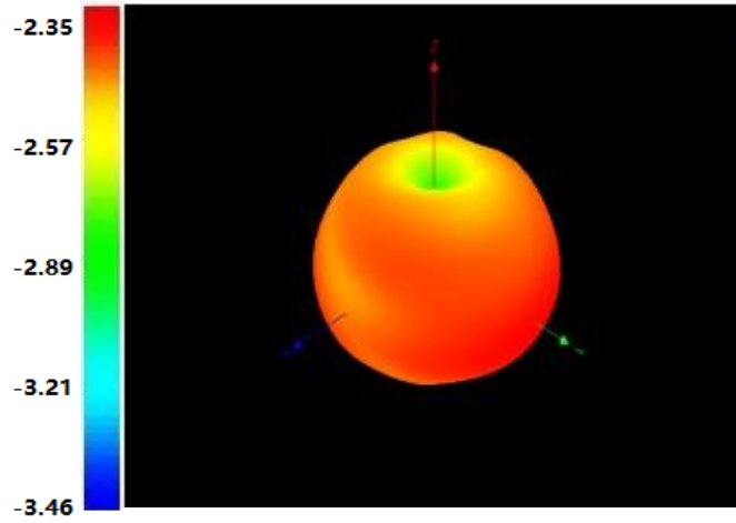
WIFI Antenna 3D Radiation Pattern
