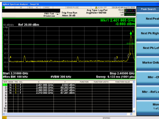
No-hopping mode
