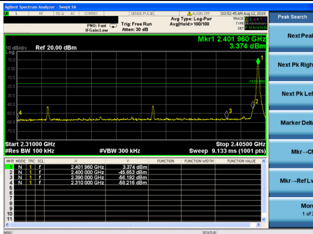
No-hopping mode
