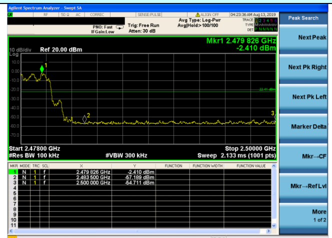
Hopping mode
