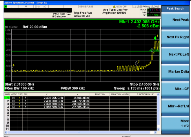
Hopping mode
