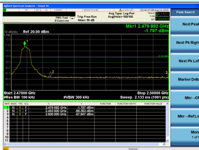
No-hopping mode
