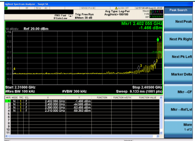
Hopping mode
