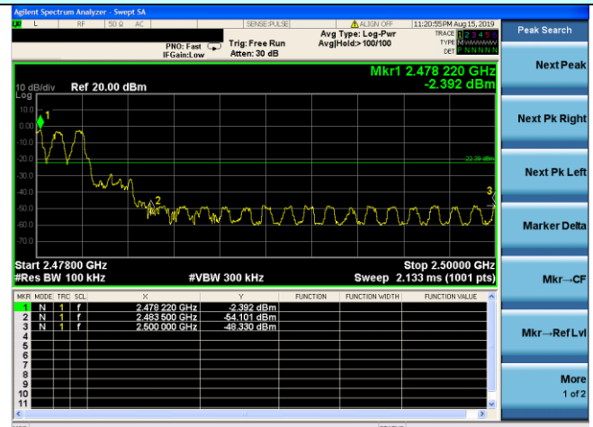
Hopping mode
