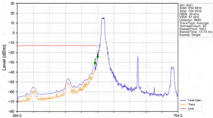
Band12_5MHz_16QAM_LCH_701.5MHz_RB_1_0_NTNV
