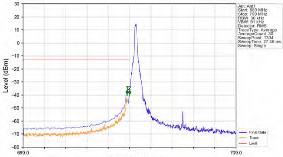
Band12_10MHz_64QAM_LCH_704MHz_RB_1_0_NTNV
