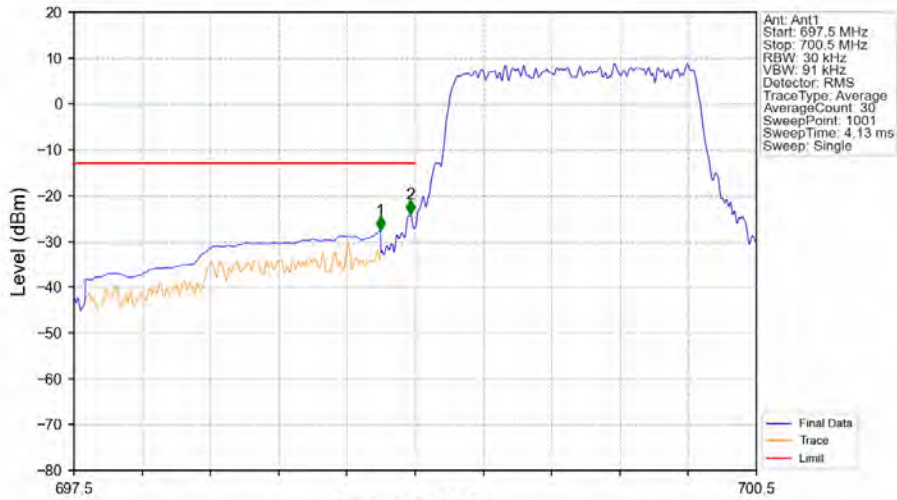
Band12_1.4MHz_QPSK_LCH_699.7MHz_RB_6_0_NTNV
