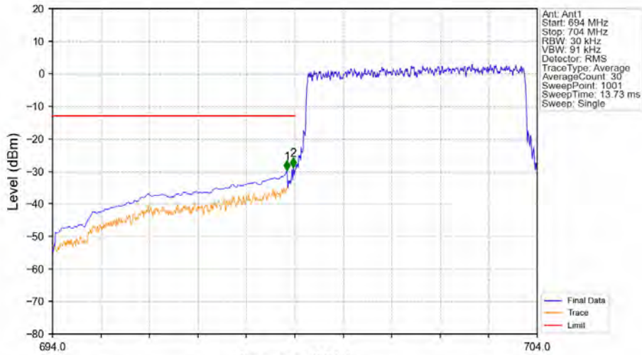
Band12_5MHz_QPSK_LCH_701.5MHz_RB_25_0_NTNV
