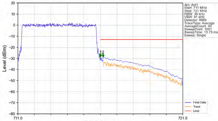
Band12_5MHz_16QAM_HCH_713.5MHz_RB_25_0_NTNV
