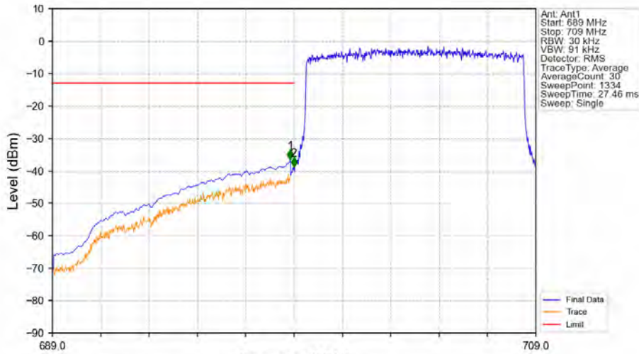
Band12_10MHz_64QAM_LCH_704MHz_RB_50_0_NTNV
