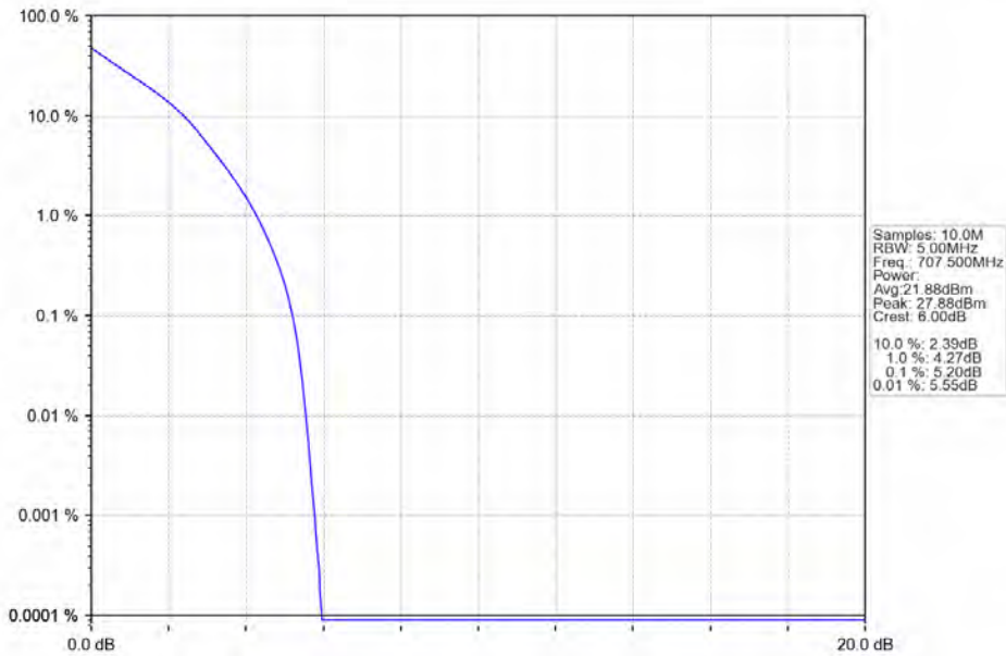
Band12_5MHz_QPSK_MCH_707.5MHz_RB_25_0_NTNV
