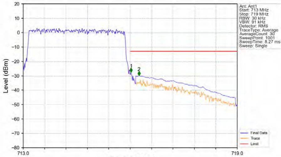
Band12_3MHz_64QAM_HCH_714.5MHz_RB_15_0_NTNV
