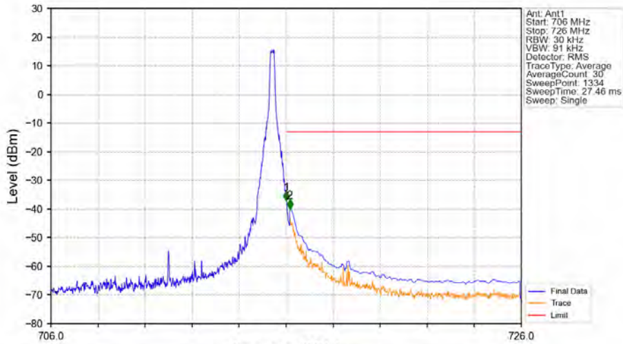
Band12_10MHz_16QAM_HCH_711MHz_RB_1_49_NTNV
