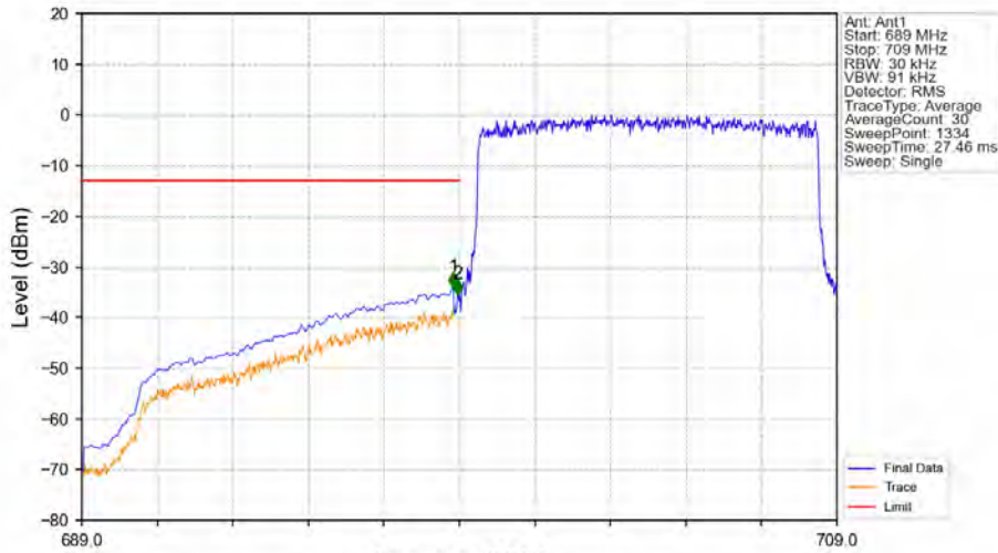
Band12_10MHz_QPSK_LCH_704MHz_RB_50_0_NTNV
