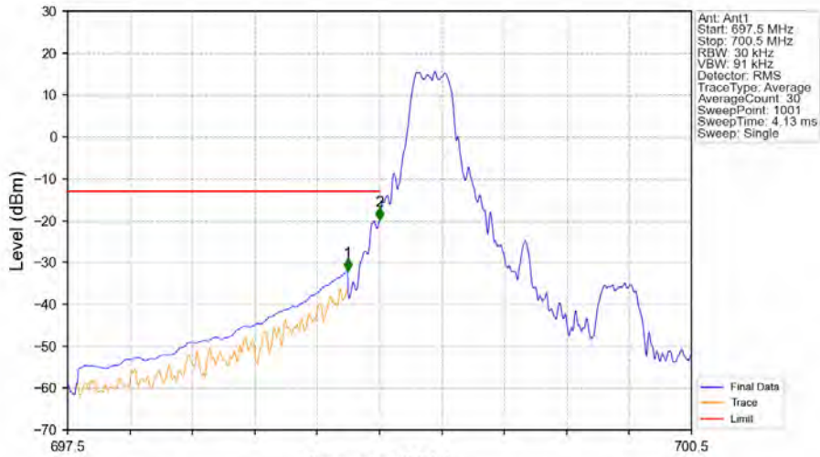
Band12_1.4MHz_16QAM_LCH_699.7MHz_RB_1_0_NTNV
