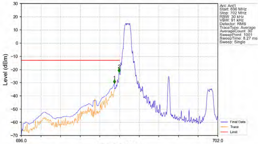
Band12_3MHz_16QAM_LCH_700.5MHz_RB_1_0_NTNV
