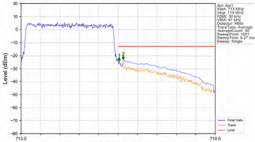
Band12_3MHz_QPSK_HCH_714.5MHz_RB_15_0_NTNV
