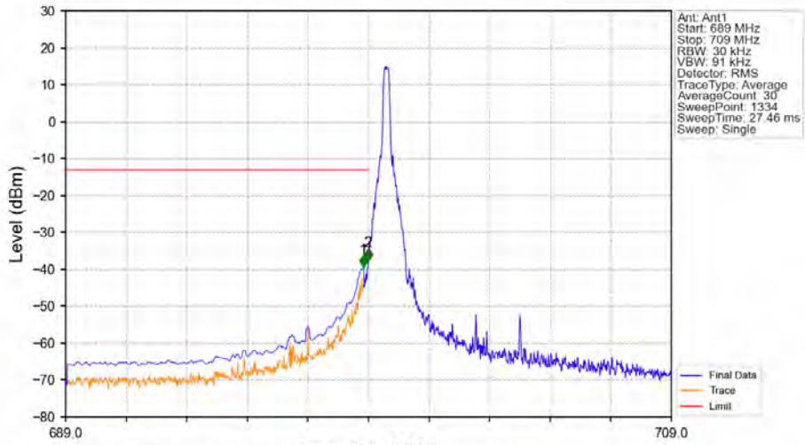
Band12_10MHz_16QAM_LCH_704MHz_RB_1_0_NTNV
