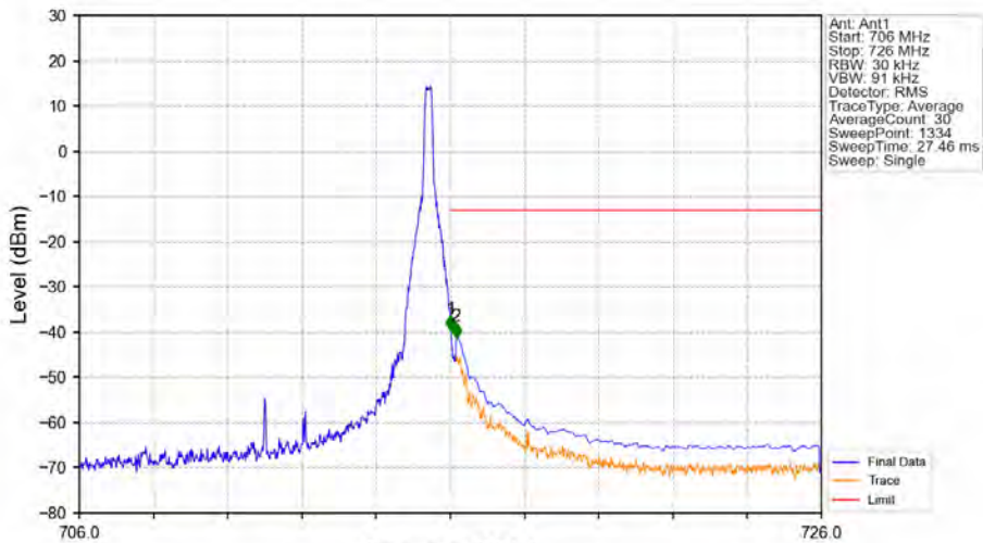
Band12_10MHz_64QAM_HCH_711MHz_RB_1_49_NTNV
