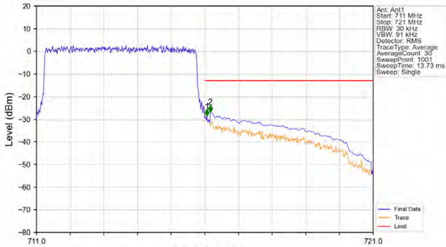
Band12_5MHz_QPSK_HCH_713.5MHz_RB_25_0_NTNV
