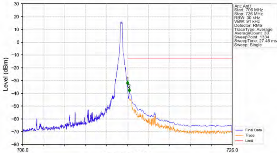
Band12_10MHz_QPSK_HCH_711MHz_RB_1_49_NTNV
