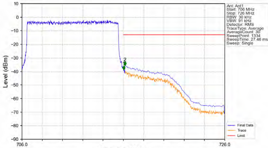
Band12_10MHz_64QAM_HCH_711MHz_RB_50_0_NTNV
