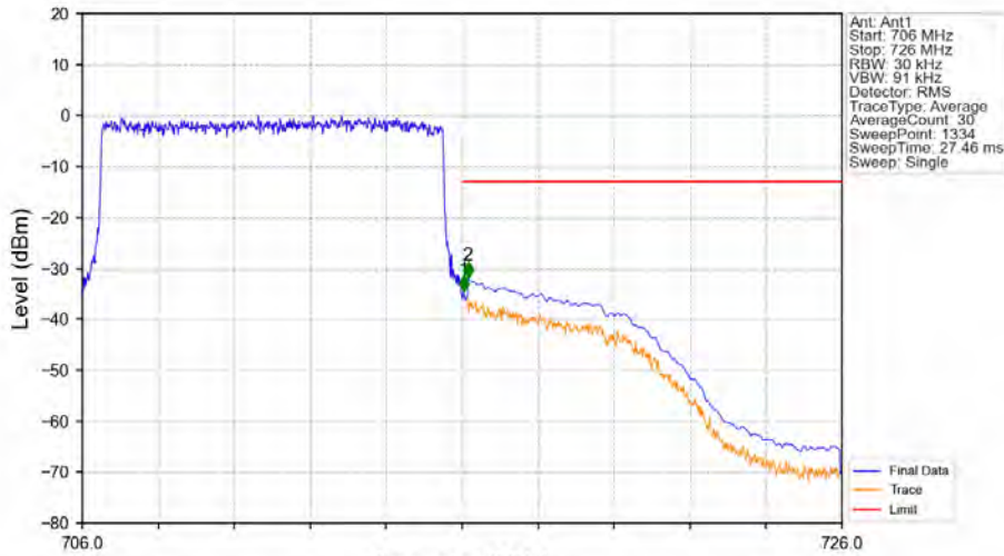
Band12_10MHz_QPSK_HCH_711MHz_RB_50_0_NTNV
