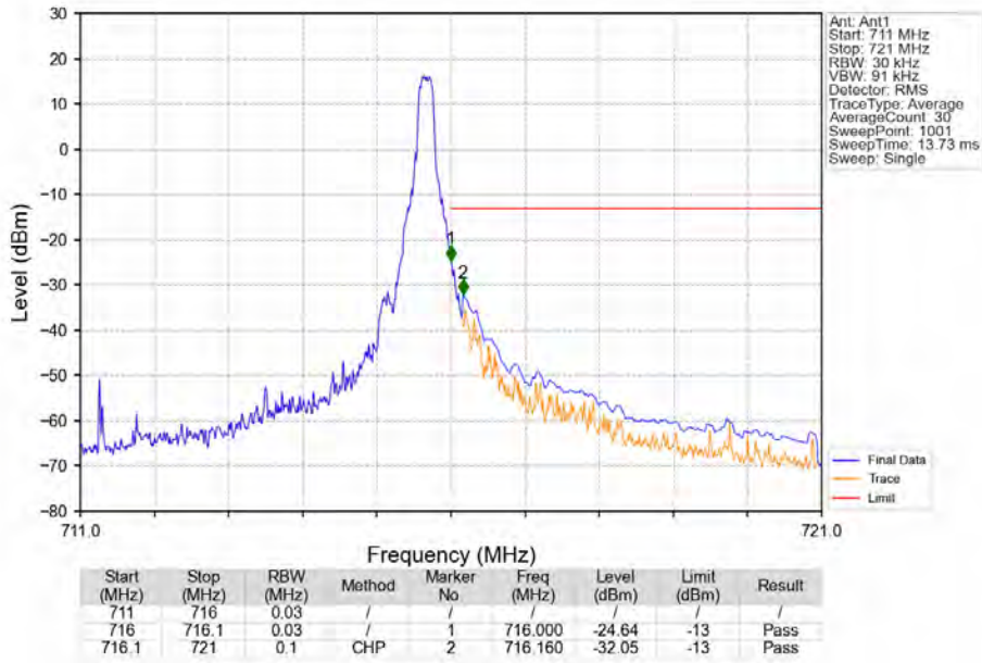
Band12_5MHz_QPSK_HCH_713.5MHz_RB_1_24_NTNV
