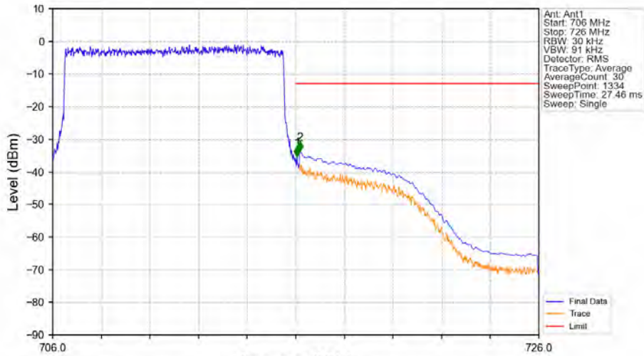
Band12_10MHz_16QAM_HCH_711MHz_RB_50_0_NTNV
