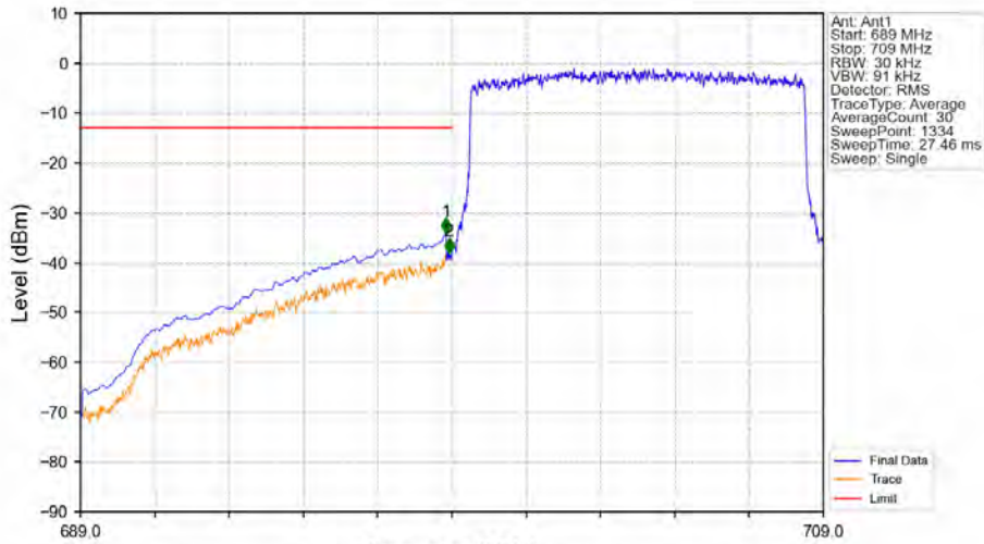
Band12_10MHz_16QAM_LCH_704MHz_RB_50_0_NTNV
