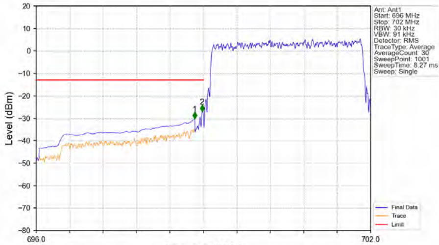
Band12_3MHz_QPSK_LCH_700.5MHz_RB_15_0_NTNV
